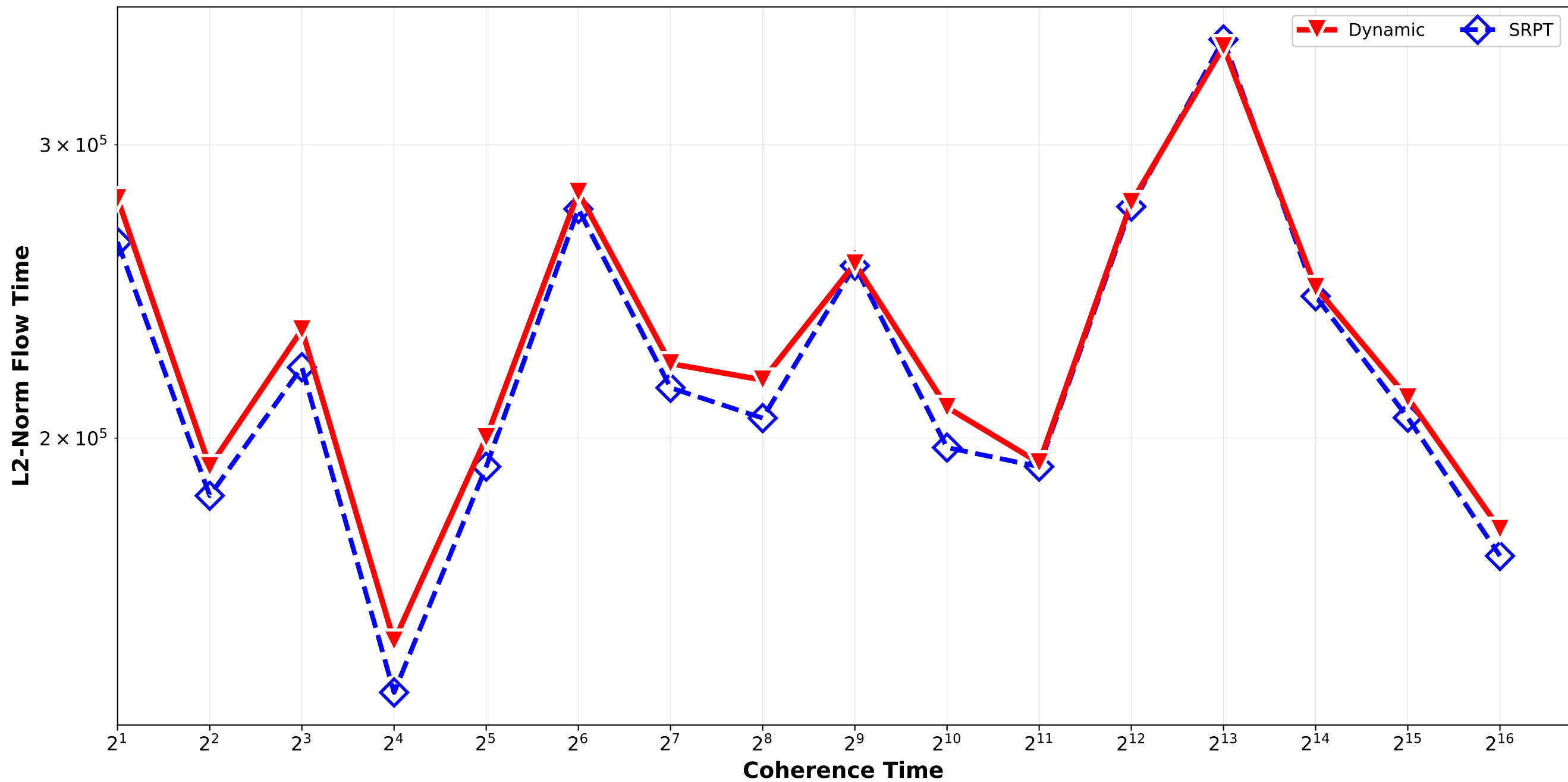
Dynamic vs SRPT - L2 Norm Flow Time Bounded_Pareto_combination_random H4096_H32768_H262144 / triplet_3
