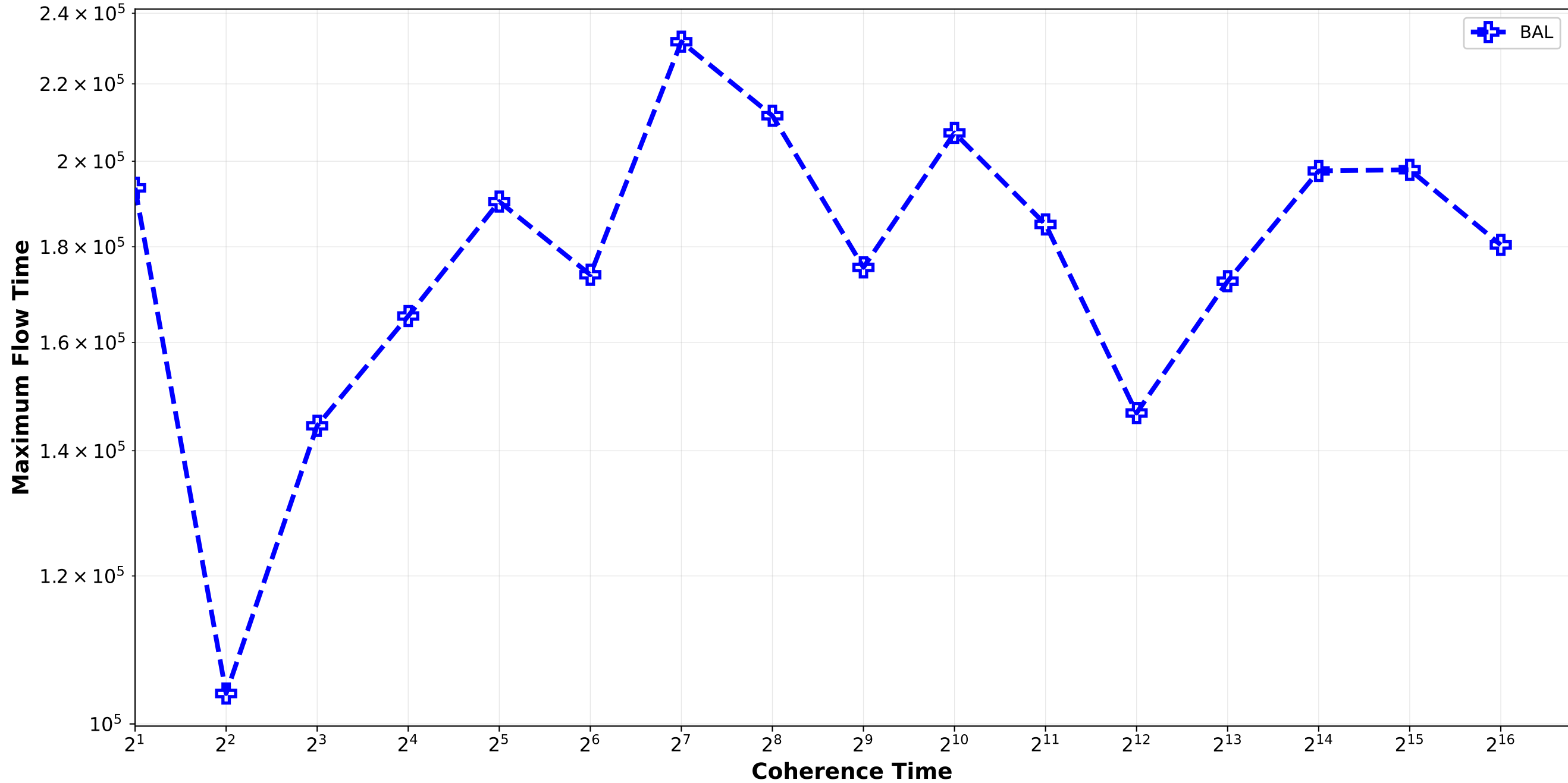
Dynamic_BAL vs BAL - Maximum Flow Time Bounded_Pareto_combination_random H512_H4096_H32768 / triplet_2
