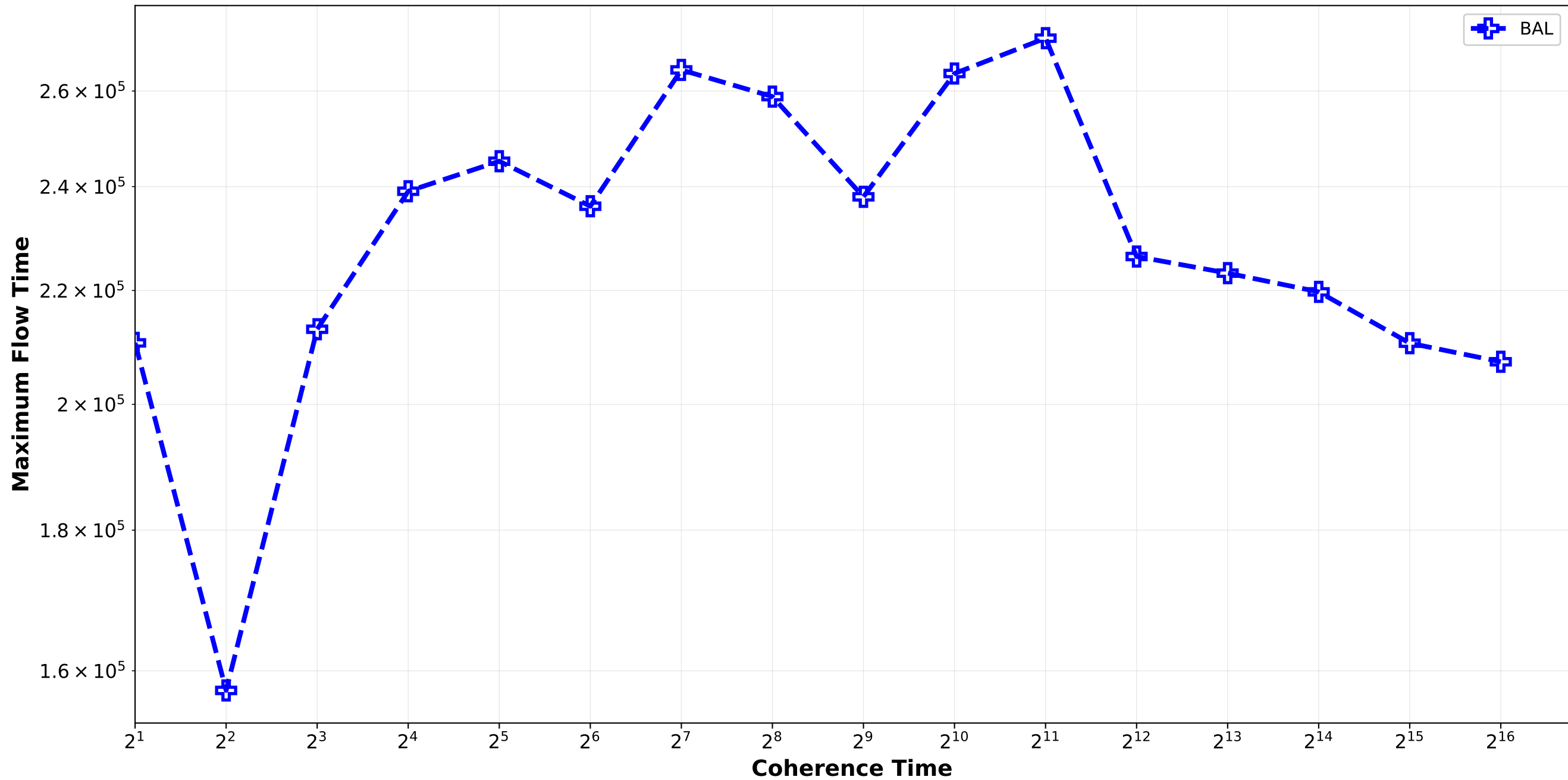
Dynamic_BAL vs BAL - Maximum Flow Time Bounded_Pareto_combination_random H64_H512_H4096 / triplet_1
