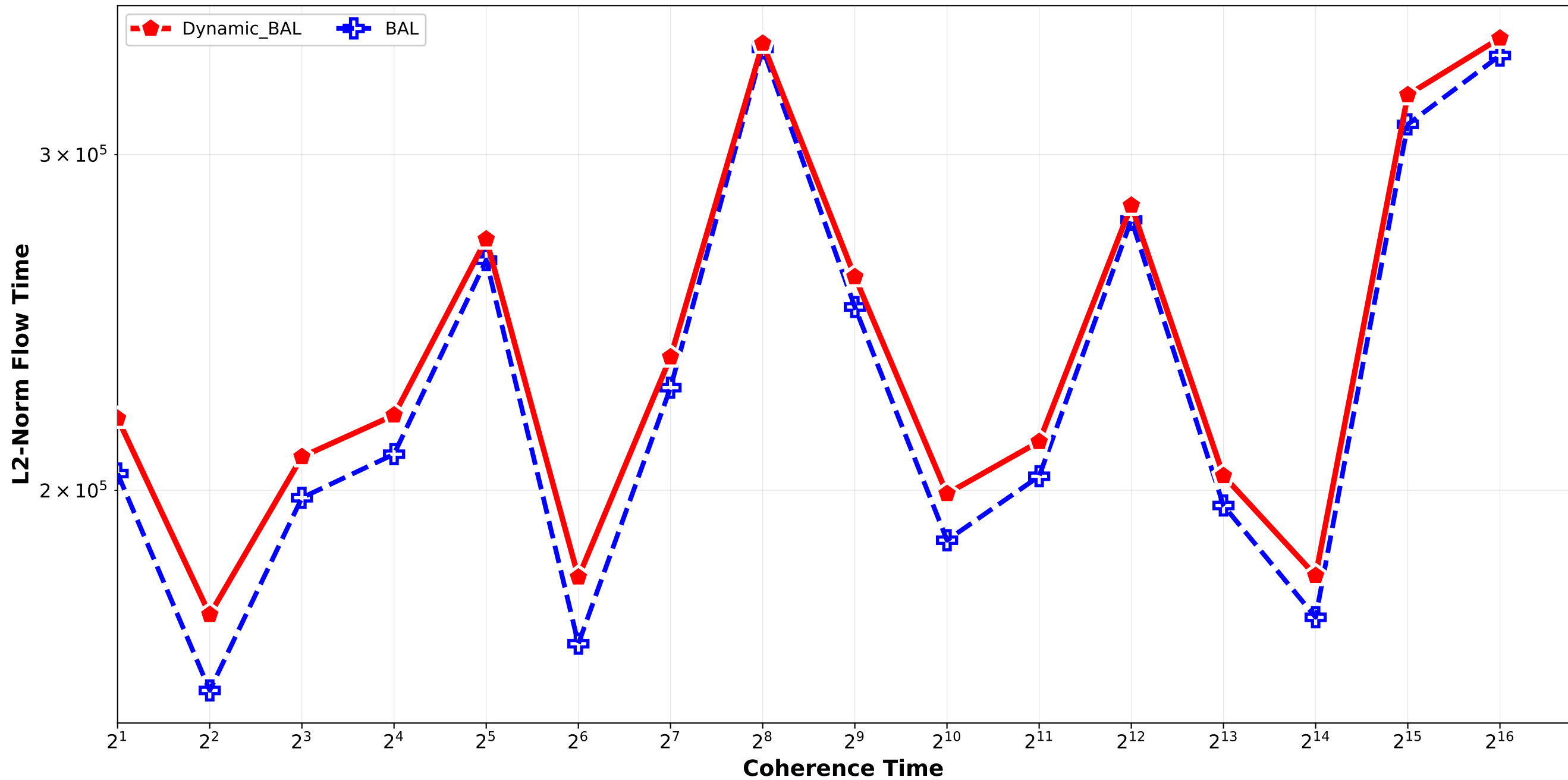
Dynamic_BAL vs BAL - L2 Norm Flow Time Bounded_Pareto_combination_random H32768_H262144 / pair_4
