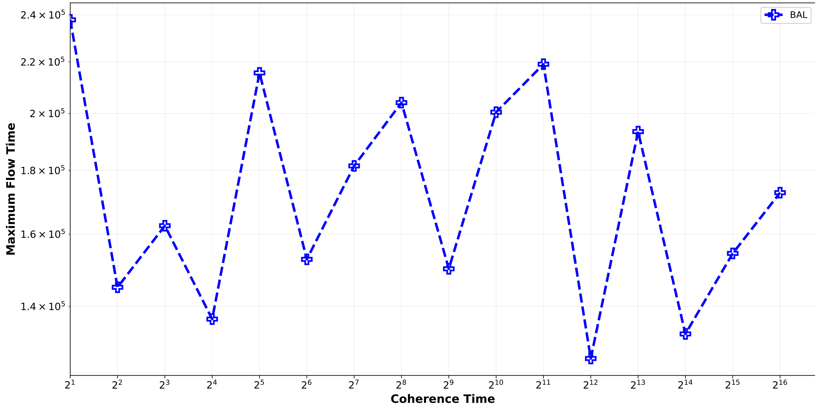
Dynamic_BAL vs BAL - Maximum Flow Time Bounded_Pareto_combination_random H4096_H32768 / pair_3
