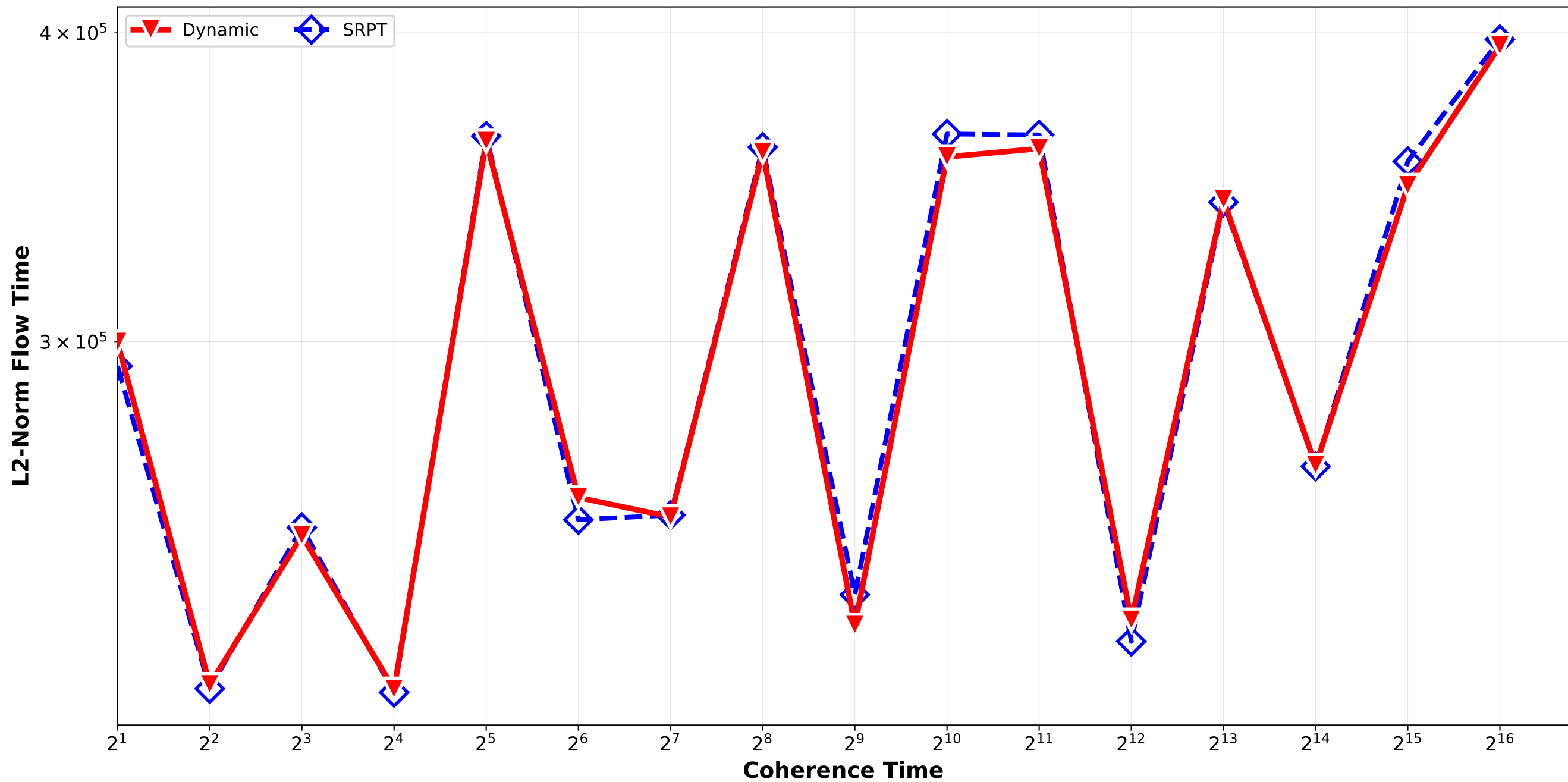
Dynamic vs SRPT - L2 Norm Flow Time Bounded_Pareto_combination_random H4096_H32768 / pair_3
