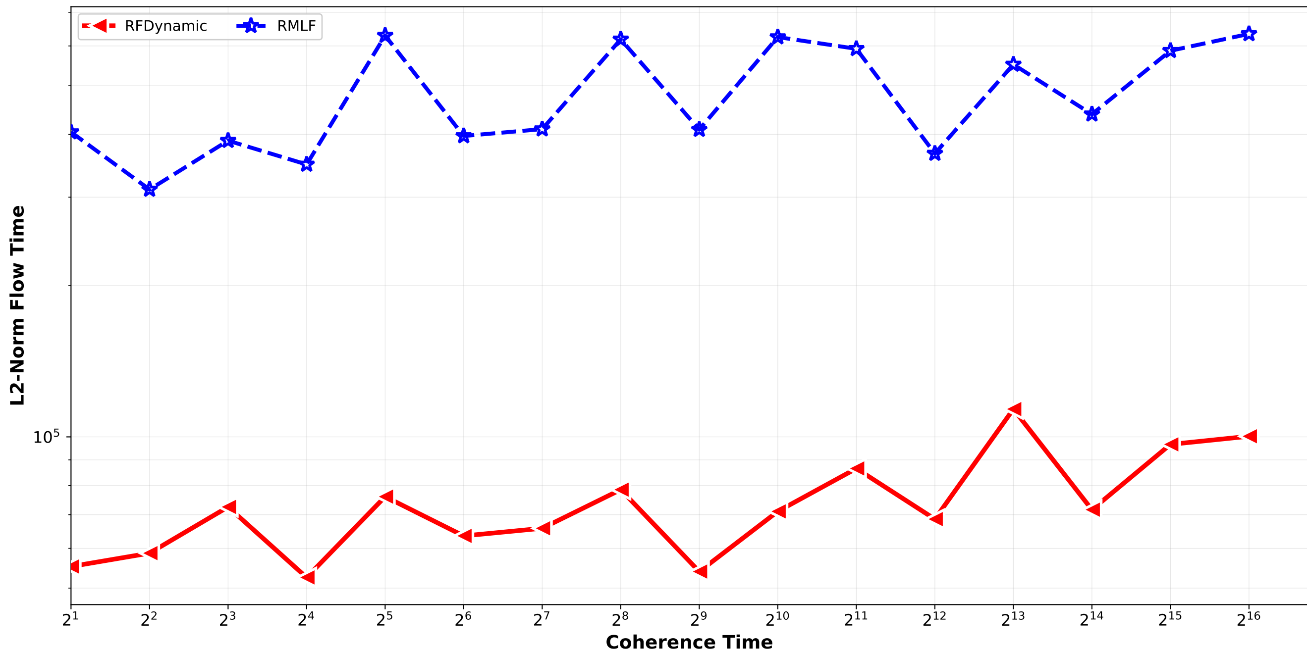
RFDynamic vs RMLF- L2 Norm Flow Time Bounded_Pareto_combination_random H4096_H32768 / pair_3
