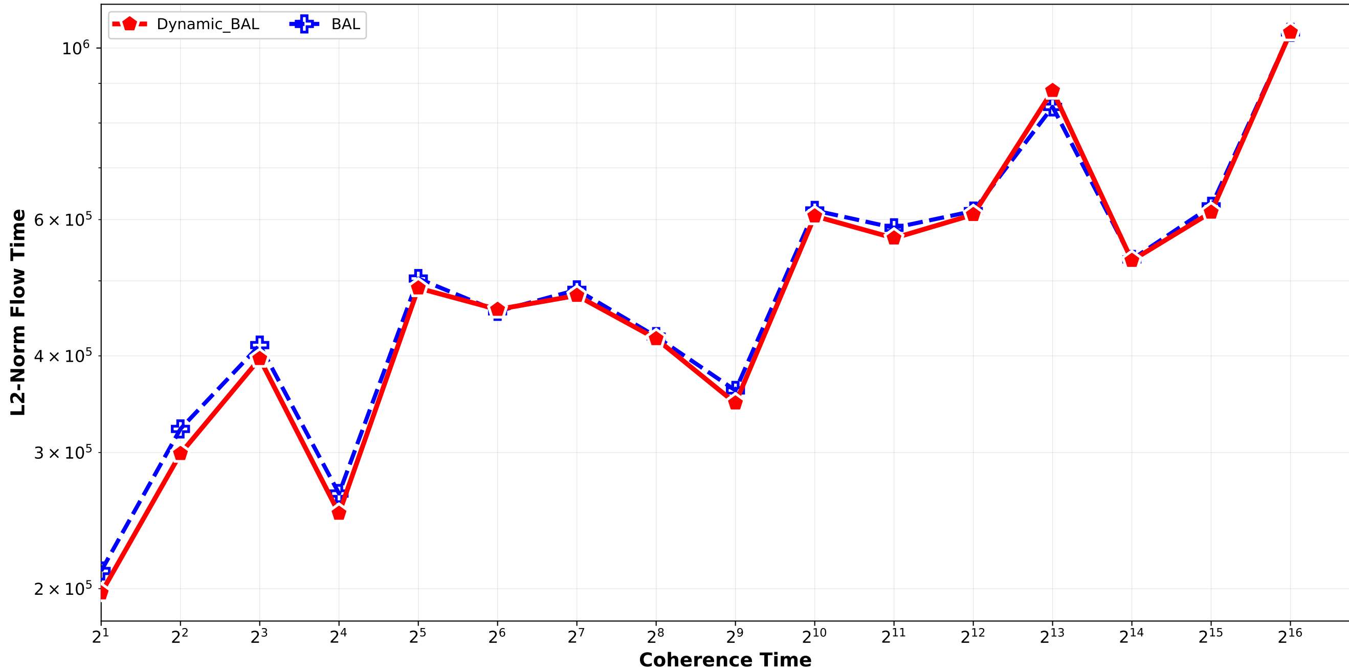
Dynamic_BAL vs BAL - L2 Norm Flow Time Bounded_Pareto_combination_random H512_H4096 / pair_2
