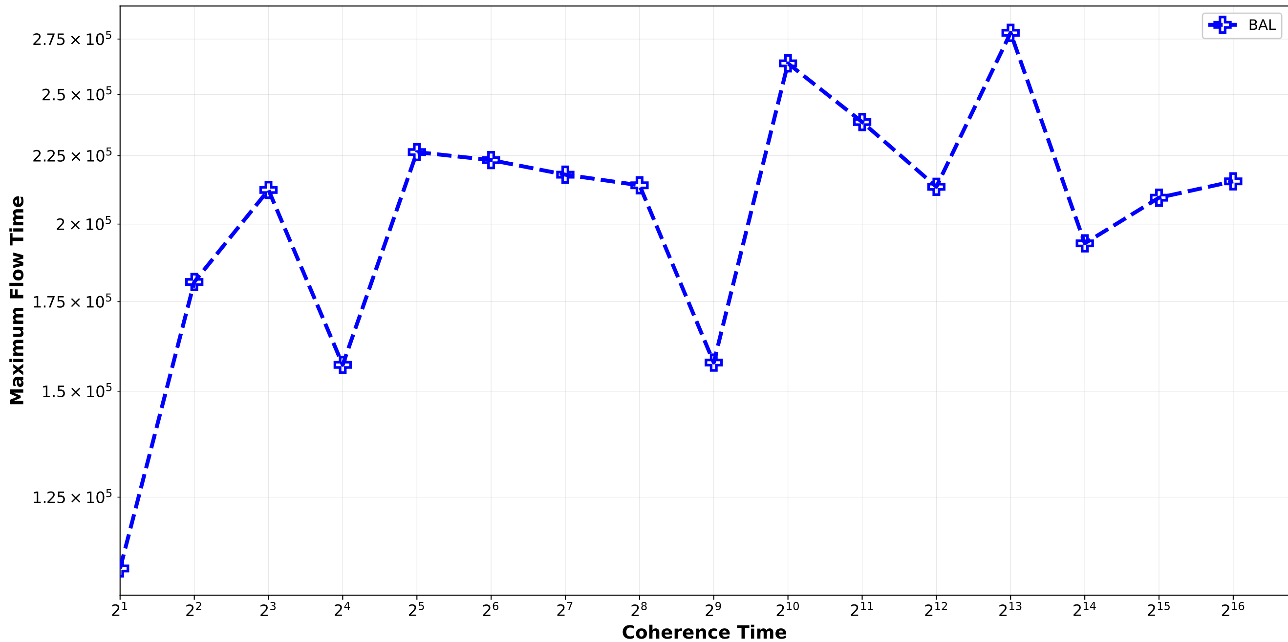
Dynamic_BAL vs BAL - Maximum Flow Time Bounded_Pareto_combination_random H512_H4096 / pair_2
