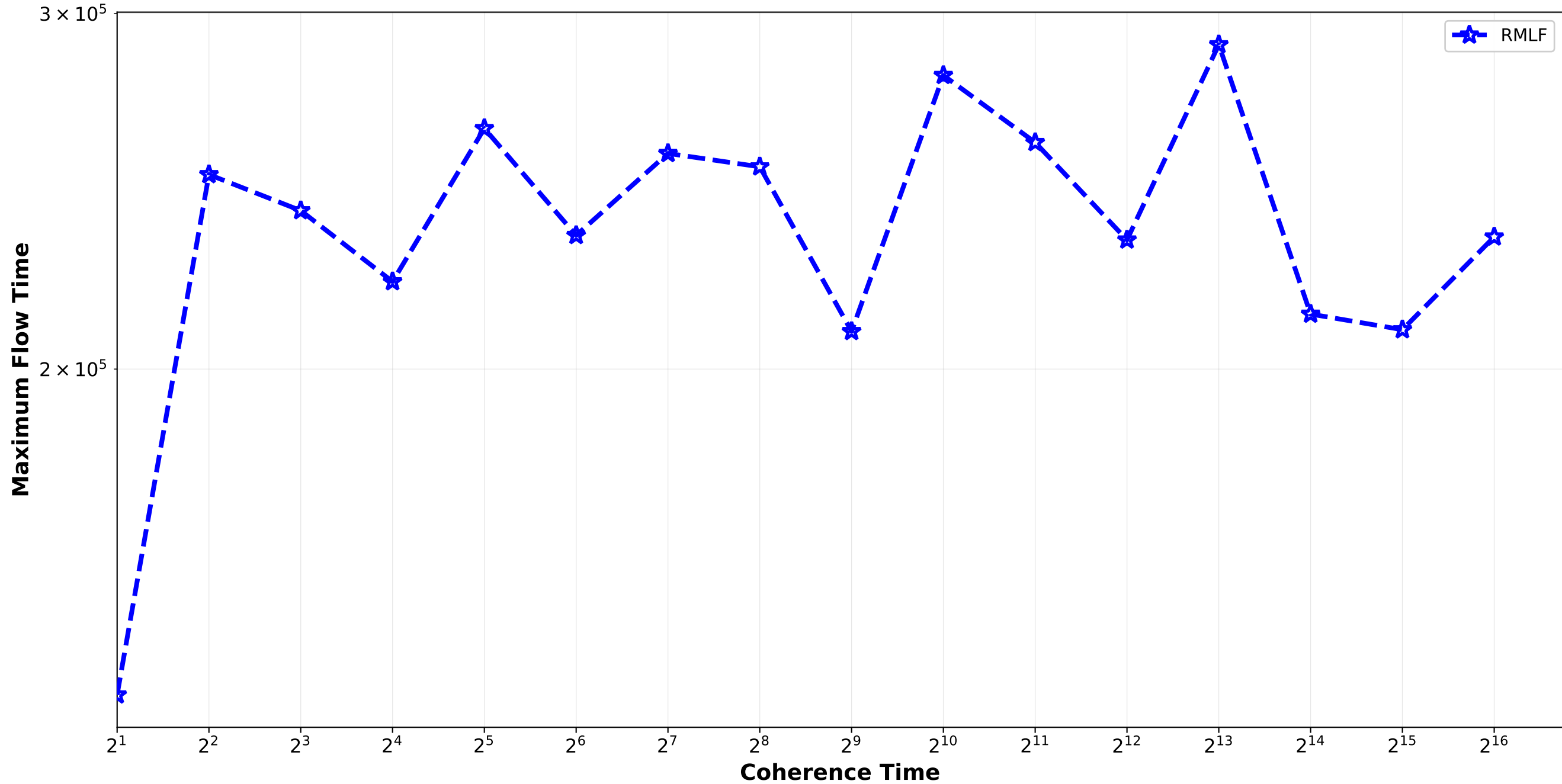
RFDynamic vs RMLF - Maximum Flow Time Bounded_Pareto_combination_random H512_H4096 / pair_2
