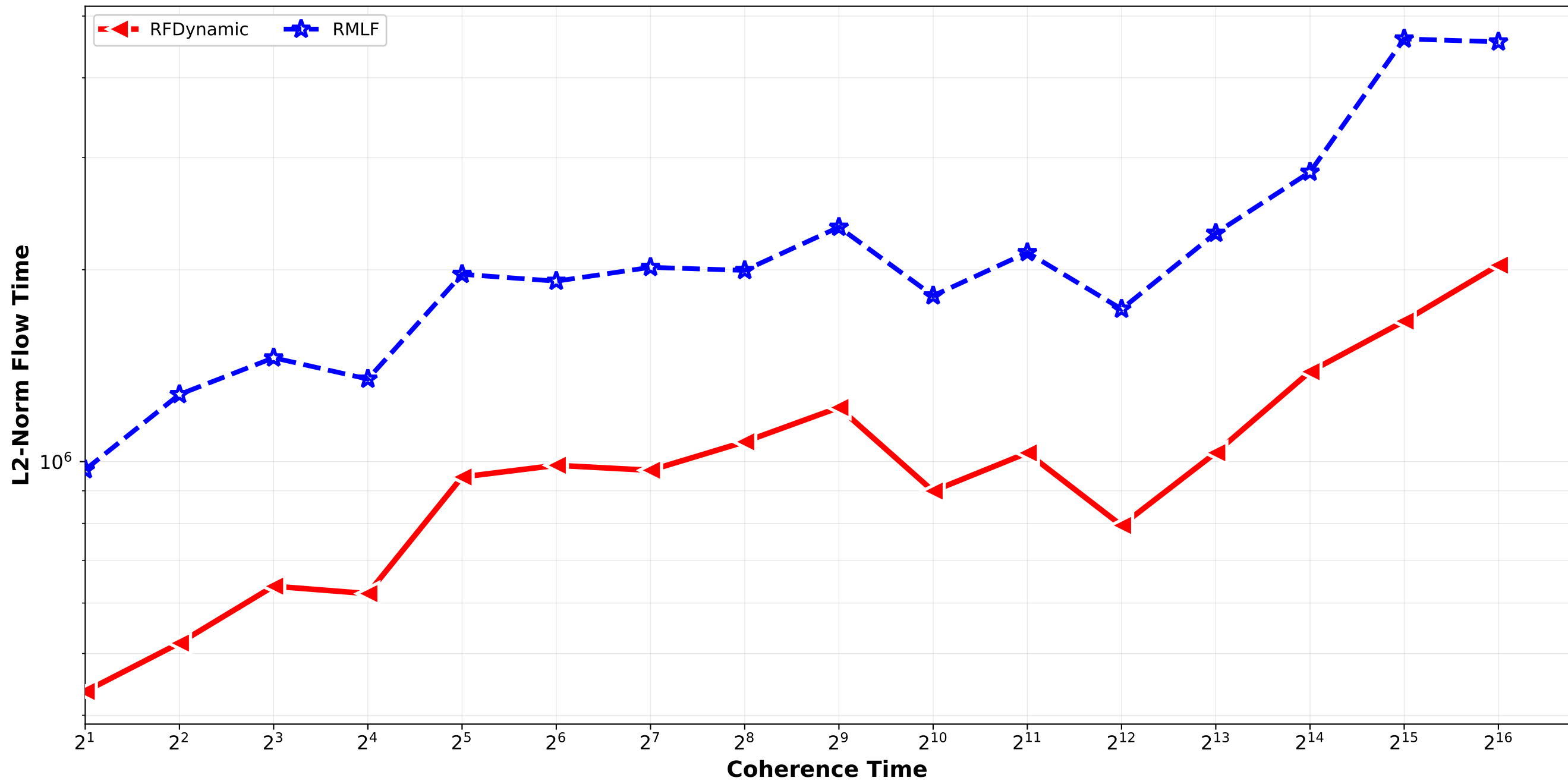
RFDynamic vs RMLF- L2 Norm Flow Time Bounded_Pareto_combination_random H64_H512 / pair_1
