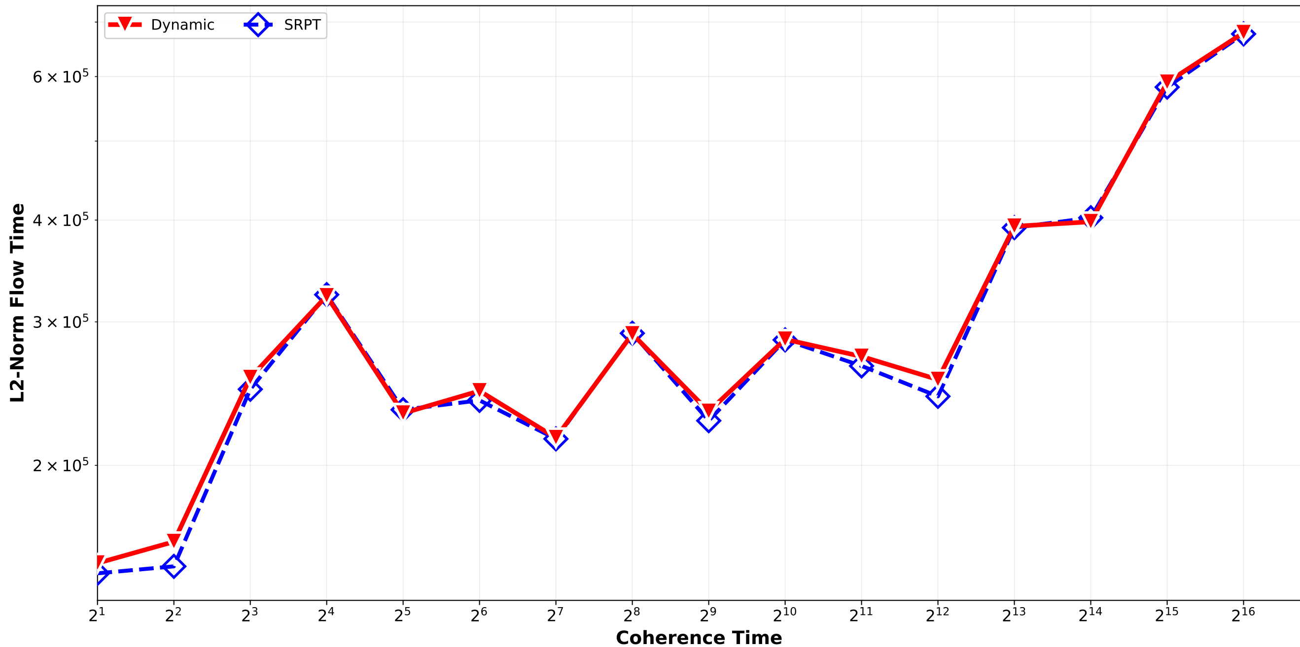
Dynamic vs SRPT - L2 Norm Flow Time Bounded_Pareto_combination_softrandom H512_H4096_H32768_H262144 / quadruplet_2
