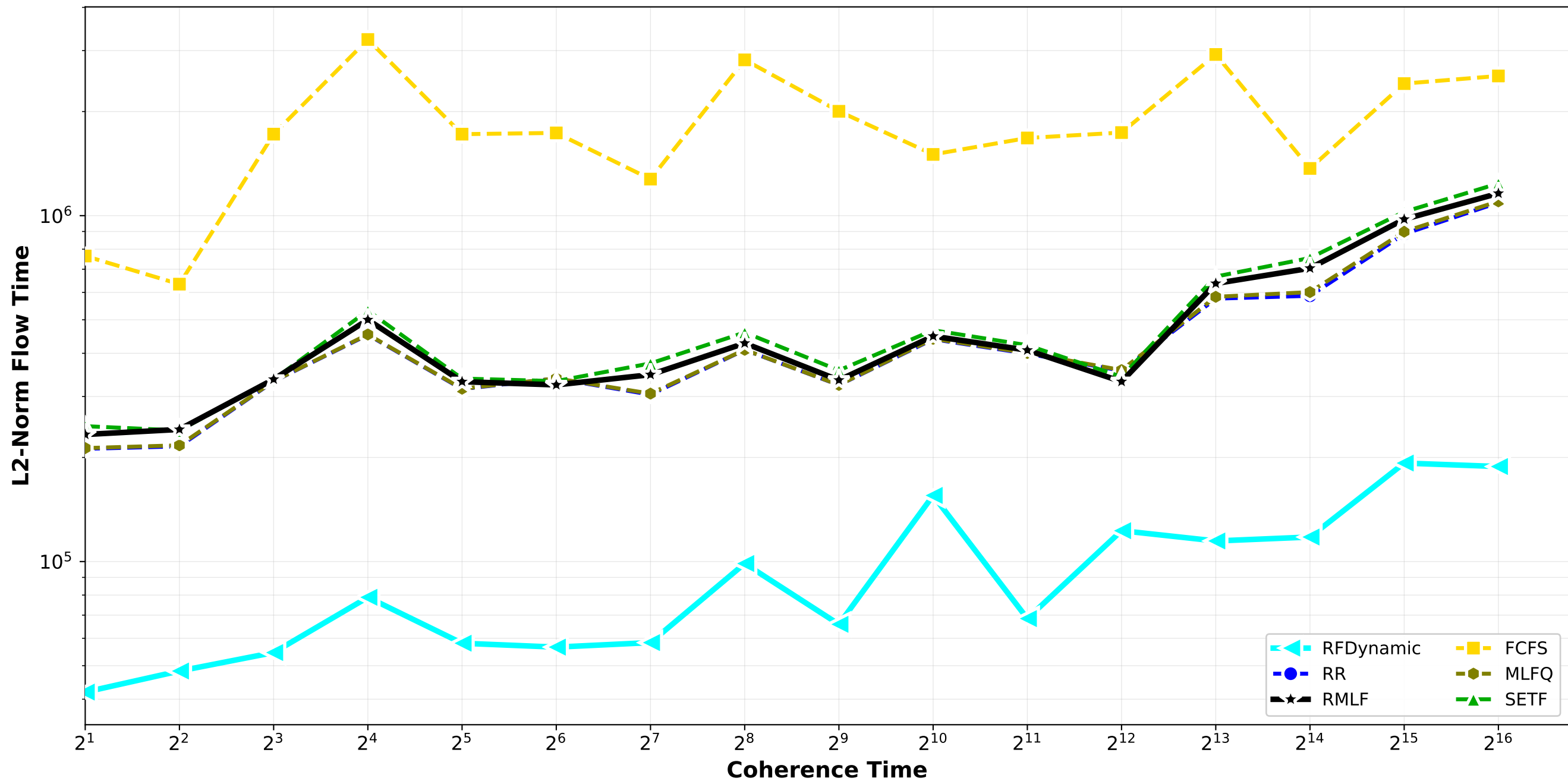
Non-Clairvoyant Algorithms - L2 Norm Flow Time Bounded_Pareto_combination_softrandom H512_H4096_H32768_H262144 / quadruplet_2
