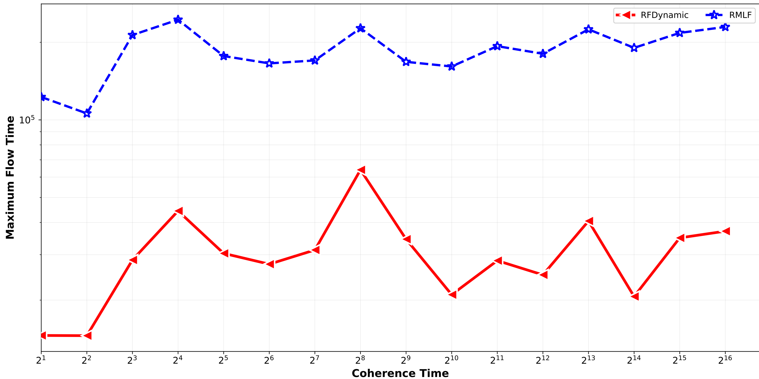
RFDynamic vs RMLF - Maximum Flow Time Bounded_Pareto_combination_softrandom H512_H4096_H32768_H262144 / quadruplet_2
