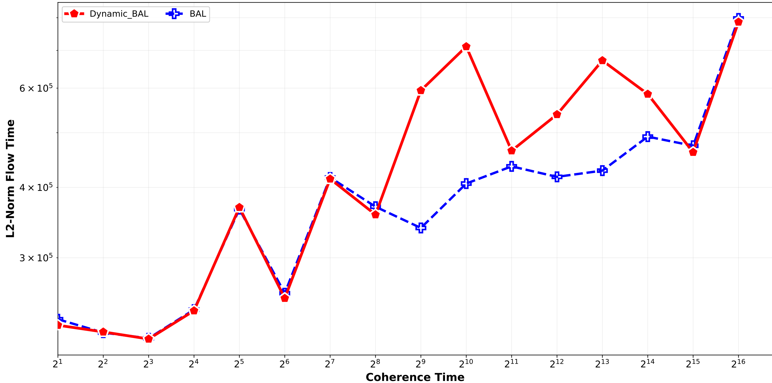
Dynamic_BAL vs BAL - L2 Norm Flow Time Bounded_Pareto_combination_softrandom H64_H512_H4096_H32768 / quadruplet_1
