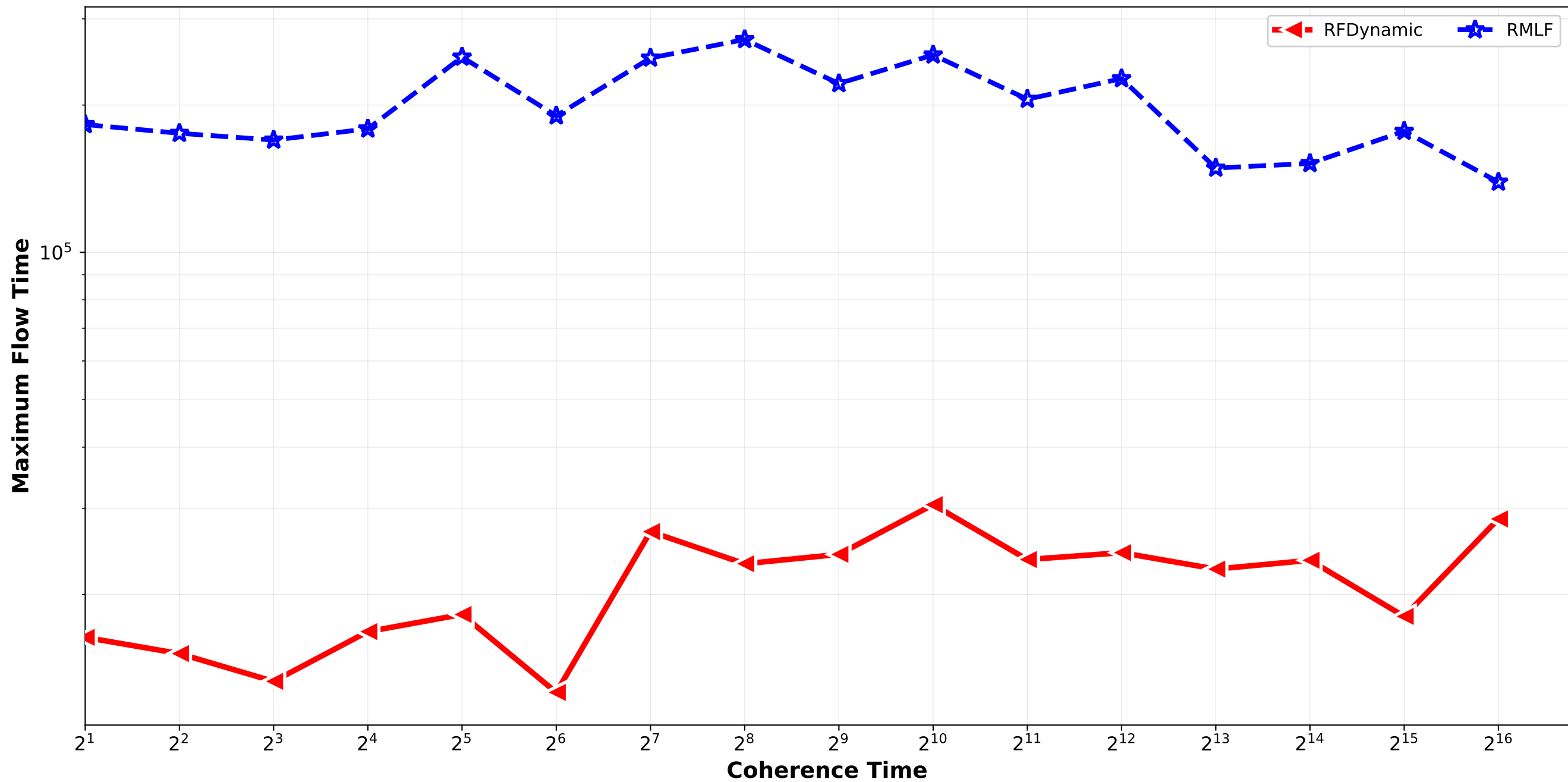
RFDynamic vs RMLF - Maximum Flow Time Bounded_Pareto_combination_softrandom H64_H512_H4096_H32768 / quadruplet_1
