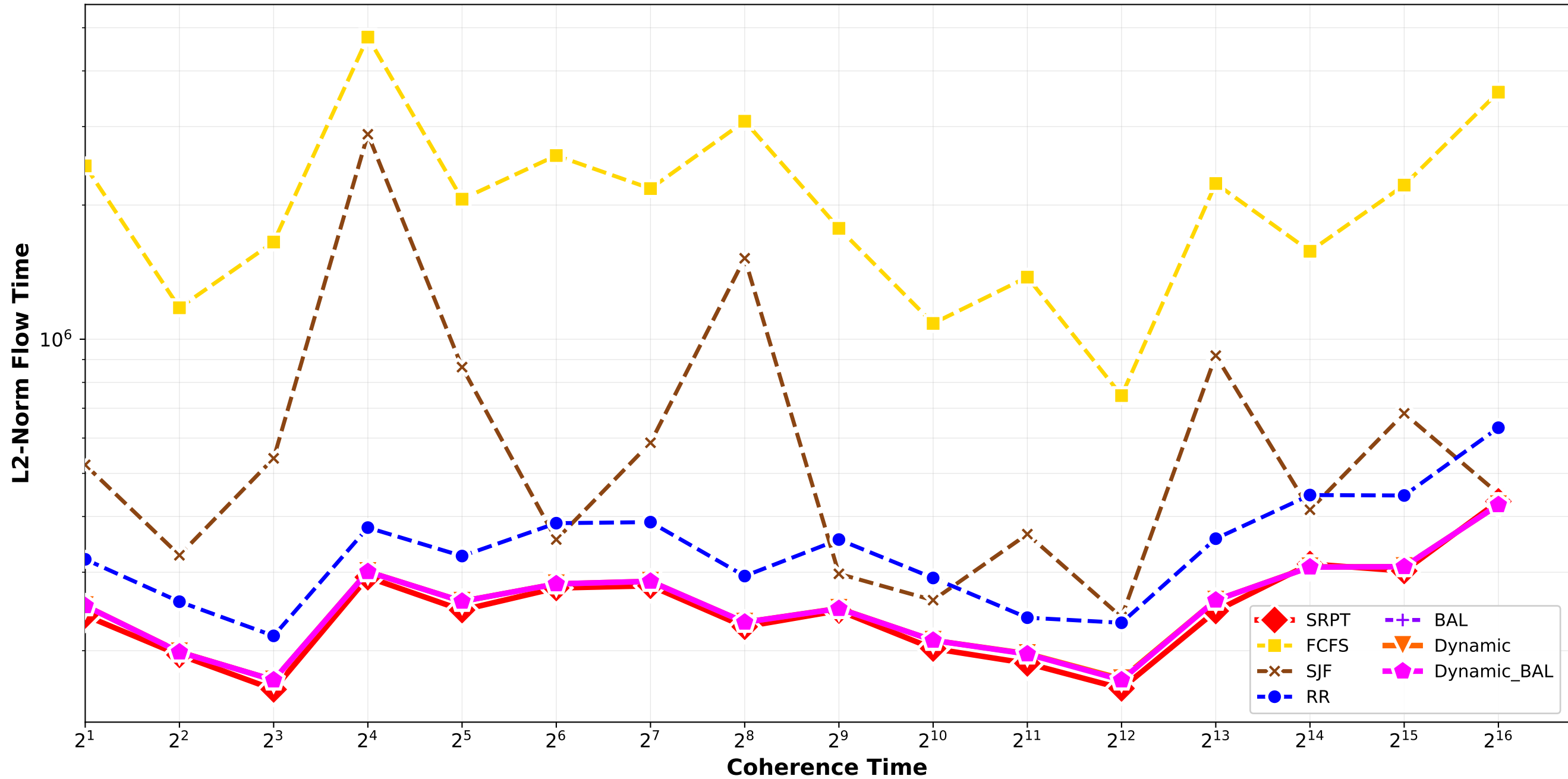
Clairvoyant Algorithms - L2 Norm Flow Time Bounded_Pareto_combination_softrandom H4096_H32768_H262144 / triplet_3
