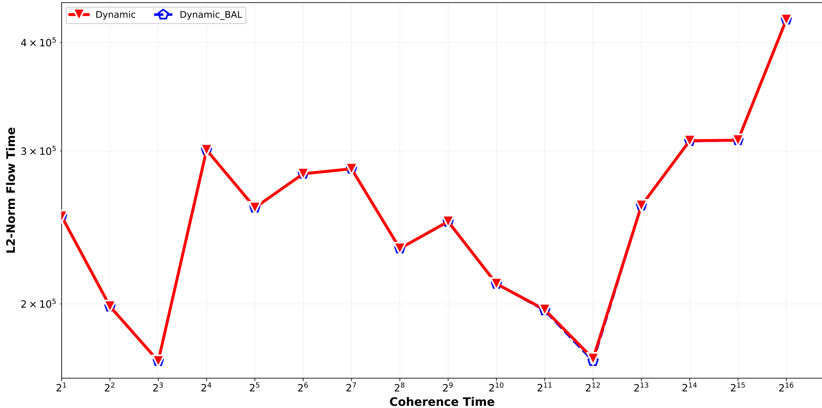
Dynamic vs Dynamic_BAL - L2 Norm Flow Time Bounded_Pareto_combination_softrandom H4096_H32768_H262144 / triplet_3
