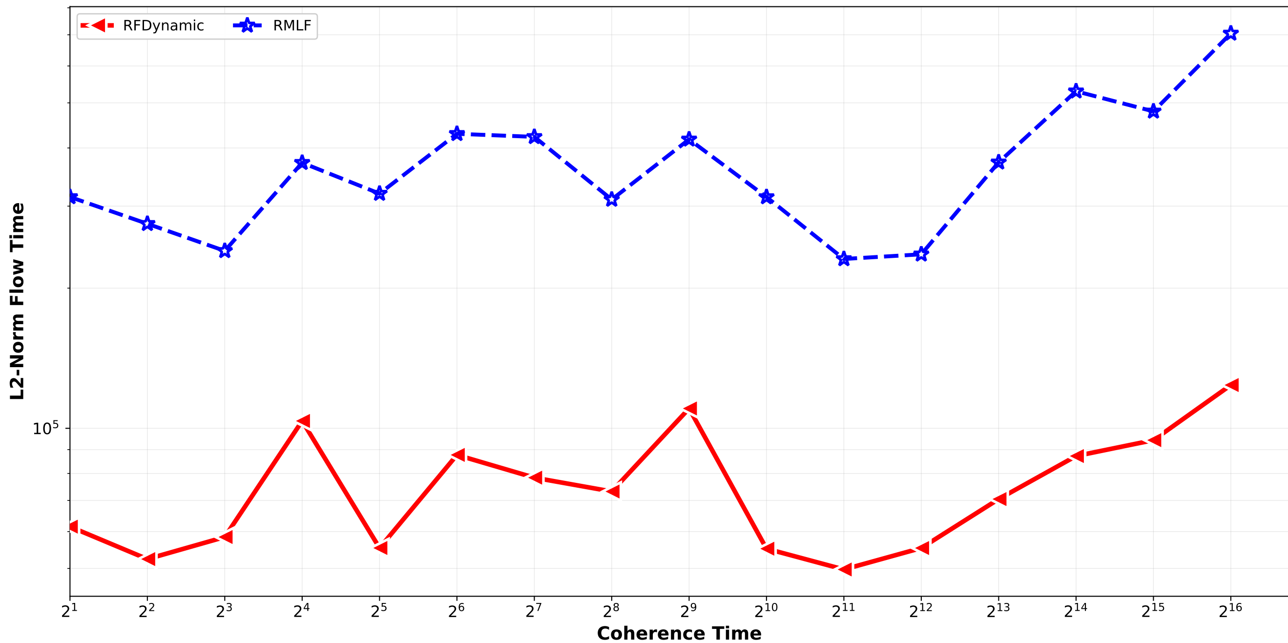
RFDynamic vs RMLF - L2 Norm Flow Time Bounded_Pareto_combination_softrandom H4096_H32768_H262144 / triplet_3
