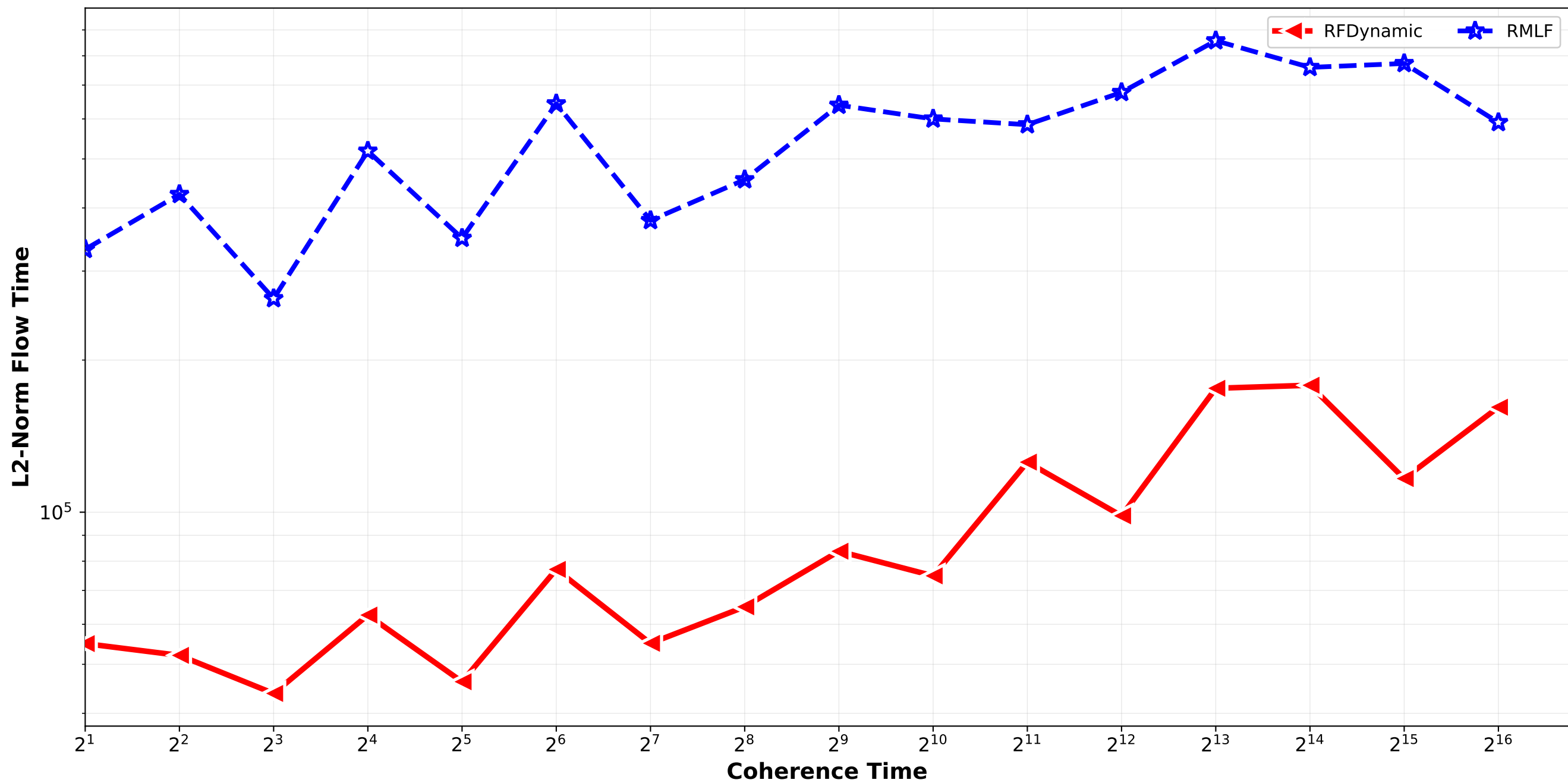
RFDynamic vs RMLF - L2 Norm Flow Time Bounded_Pareto_combination_softrandom H512_H4096_H32768 / triplet_2
