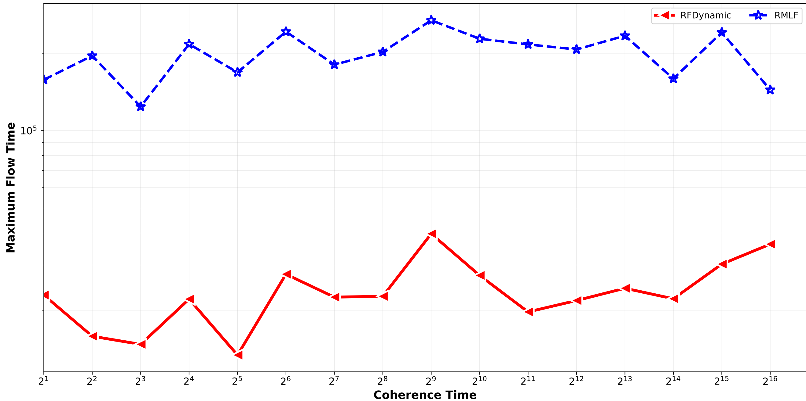
RFDynamic vs RMLF - Maximum Flow Time Bounded_Pareto_combination_softrandom H512_H4096_H32768 / triplet_2
