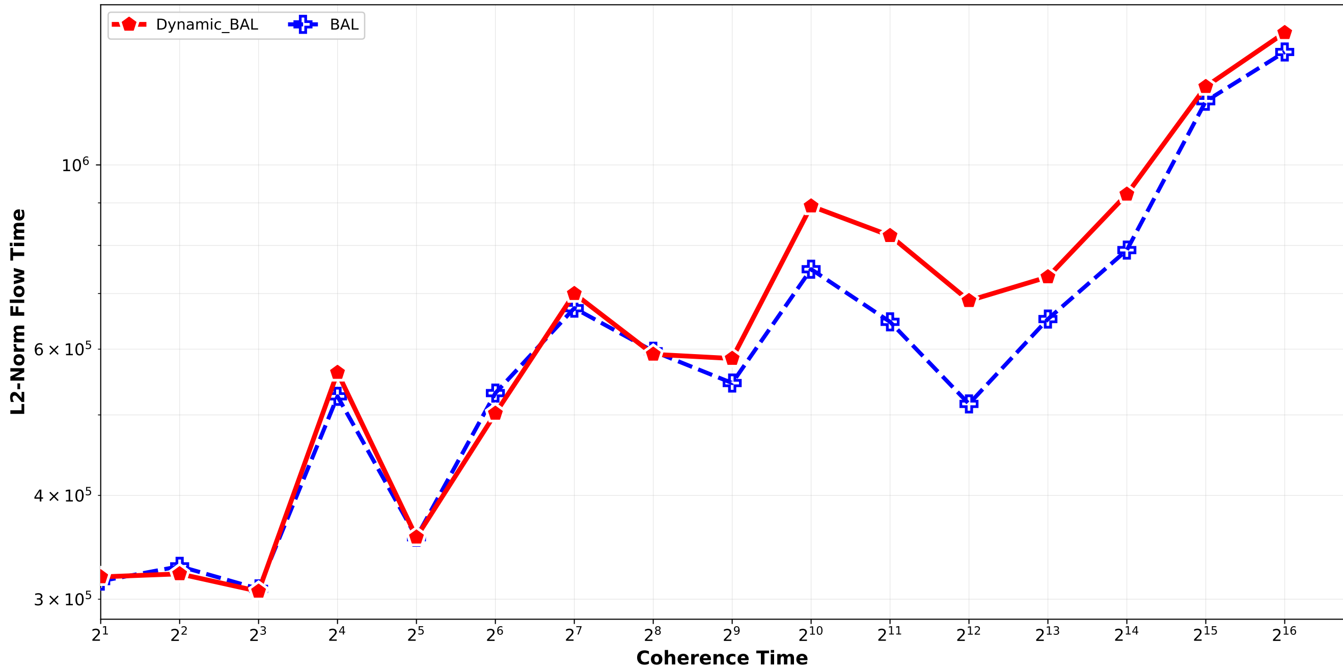
Dynamic_BAL vs BAL - L2 Norm Flow Time Bounded_Pareto_combination_softrandom H64_H512_H4096 / triplet_1
