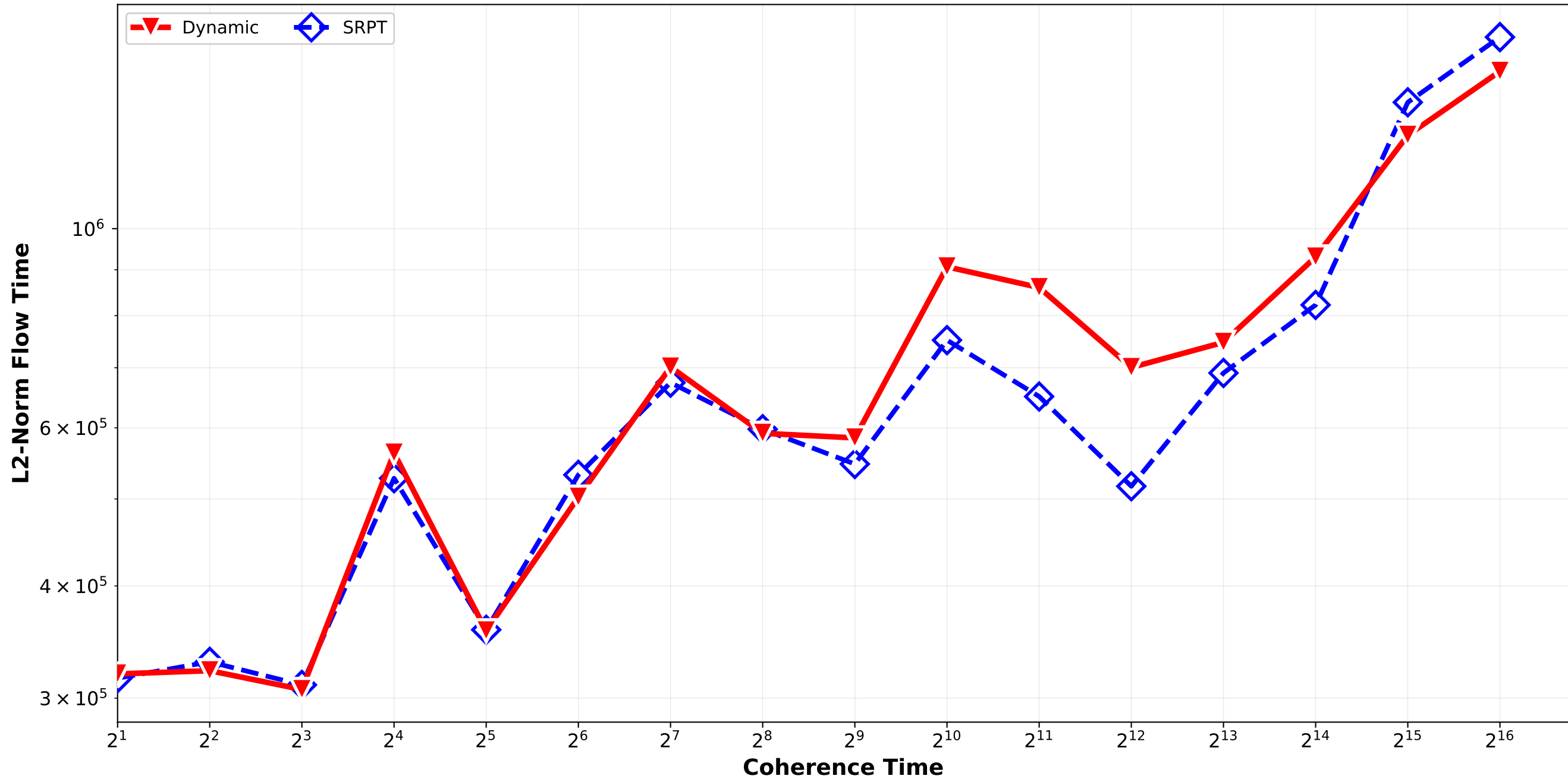
Dynamic vs SRPT - L2 Norm Flow Time Bounded_Pareto_combination_softrandom H64_H512_H4096 / triplet_1
