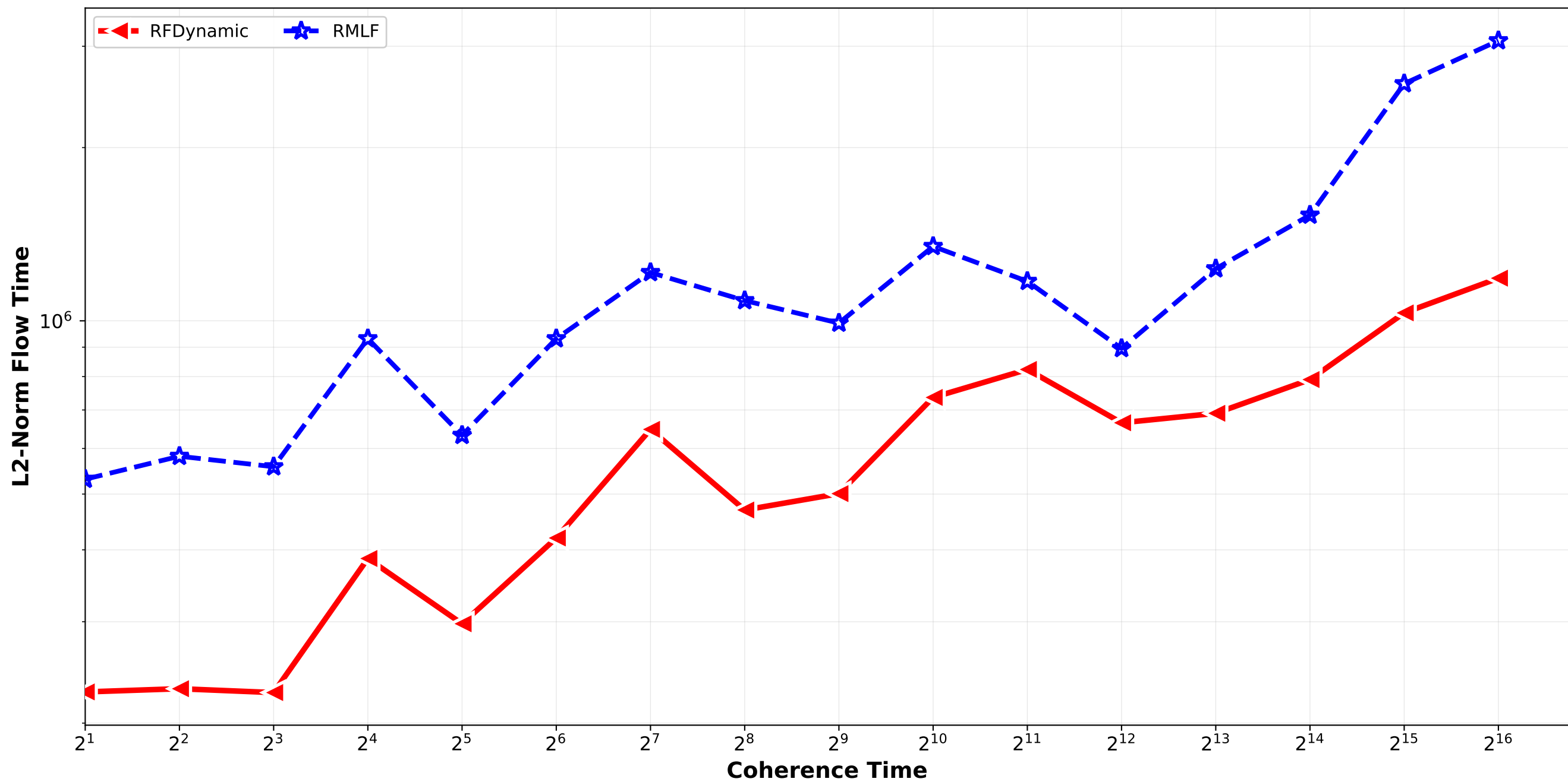
RFDynamic vs RMLF - L2 Norm Flow Time Bounded_Pareto_combination_softrandom H64_H512_H4096 / triplet_1
