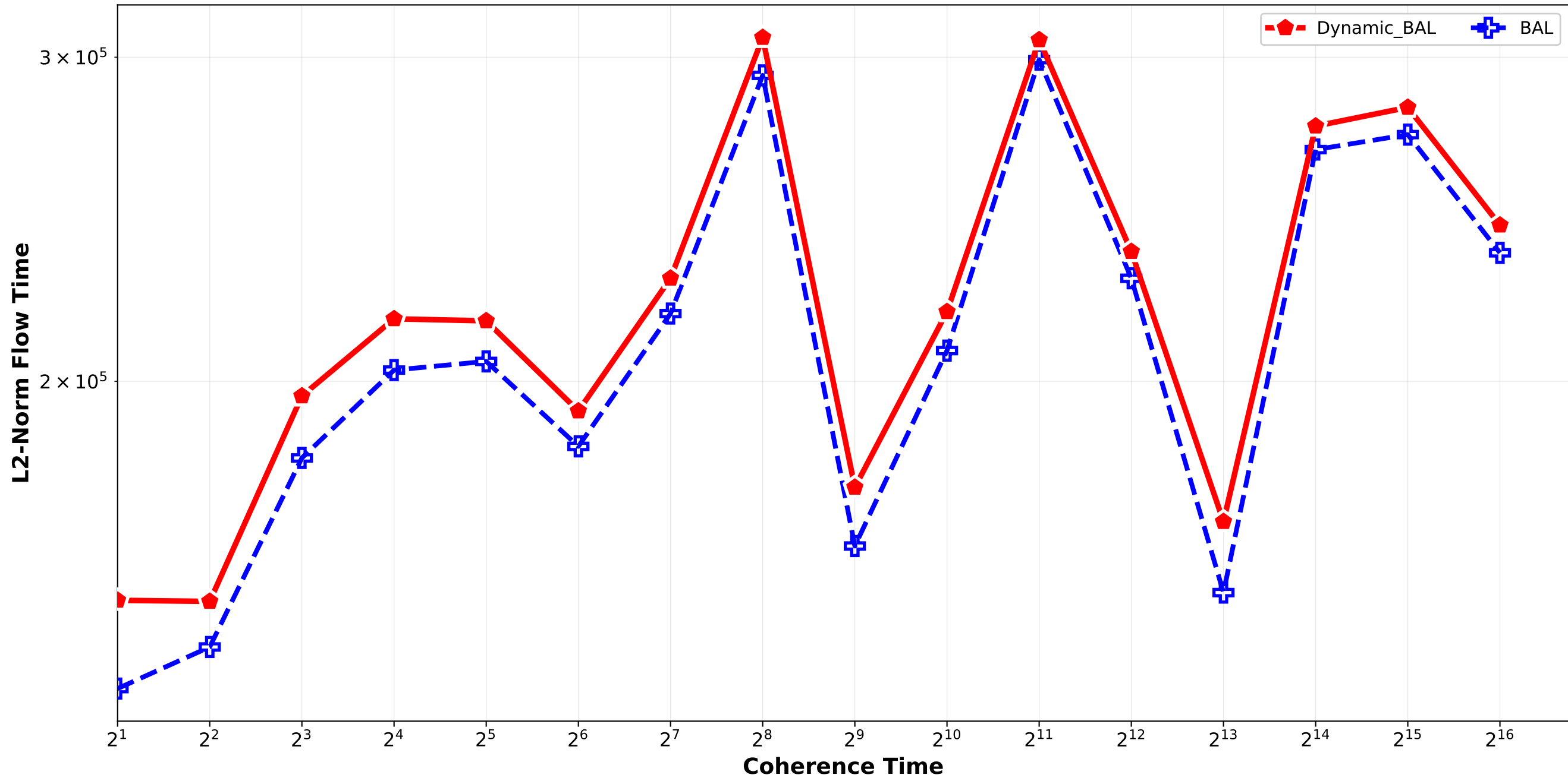
Dynamic_BAL vs BAL - L2 Norm Flow Time Bounded_Pareto_combination_softrandom H32768_H262144 / pair_4
