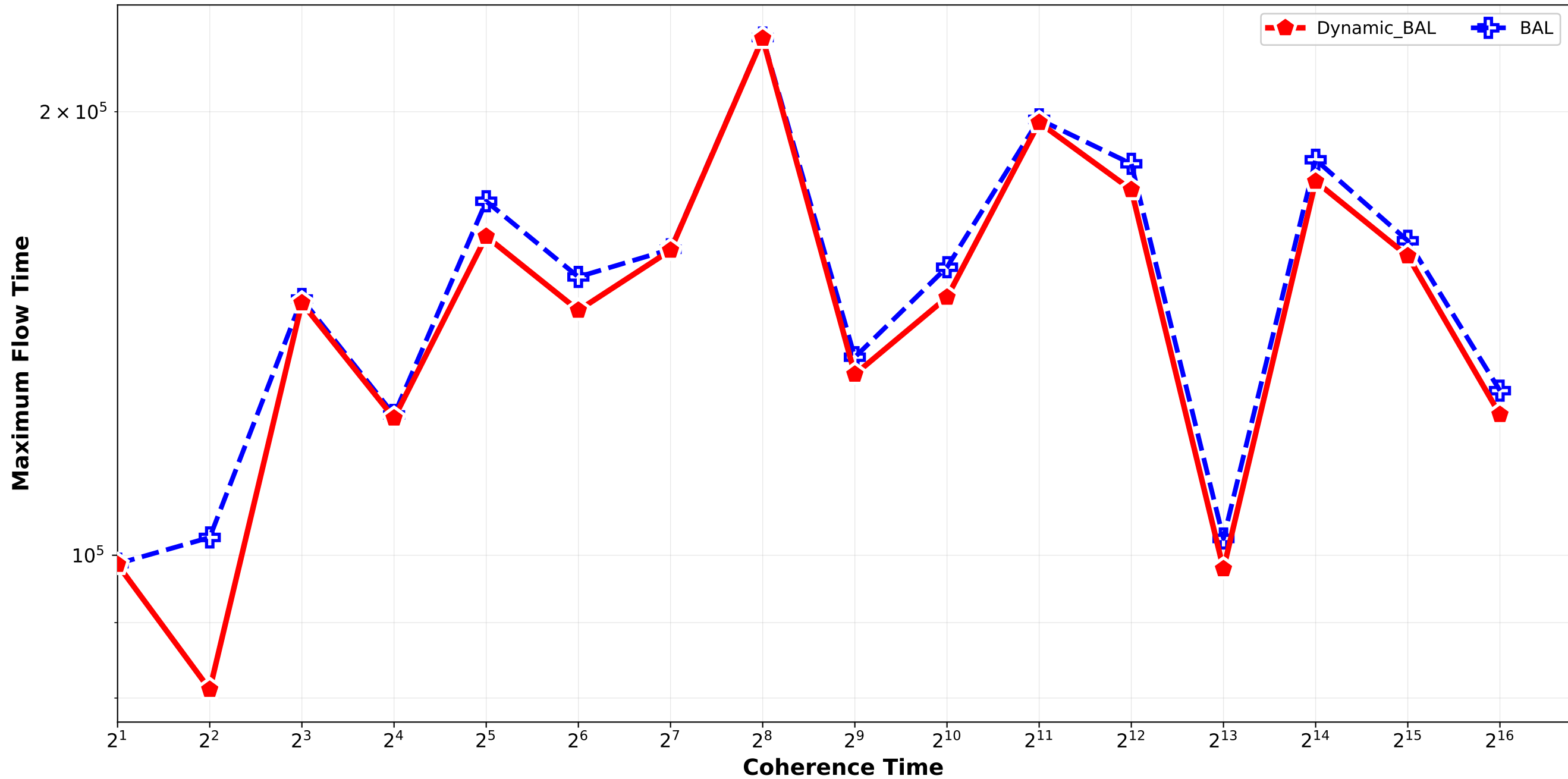
Dynamic_BAL vs BAL - Maximum Flow Time Bounded_Pareto_combination_softrandom H32768_H262144 / pair_4
