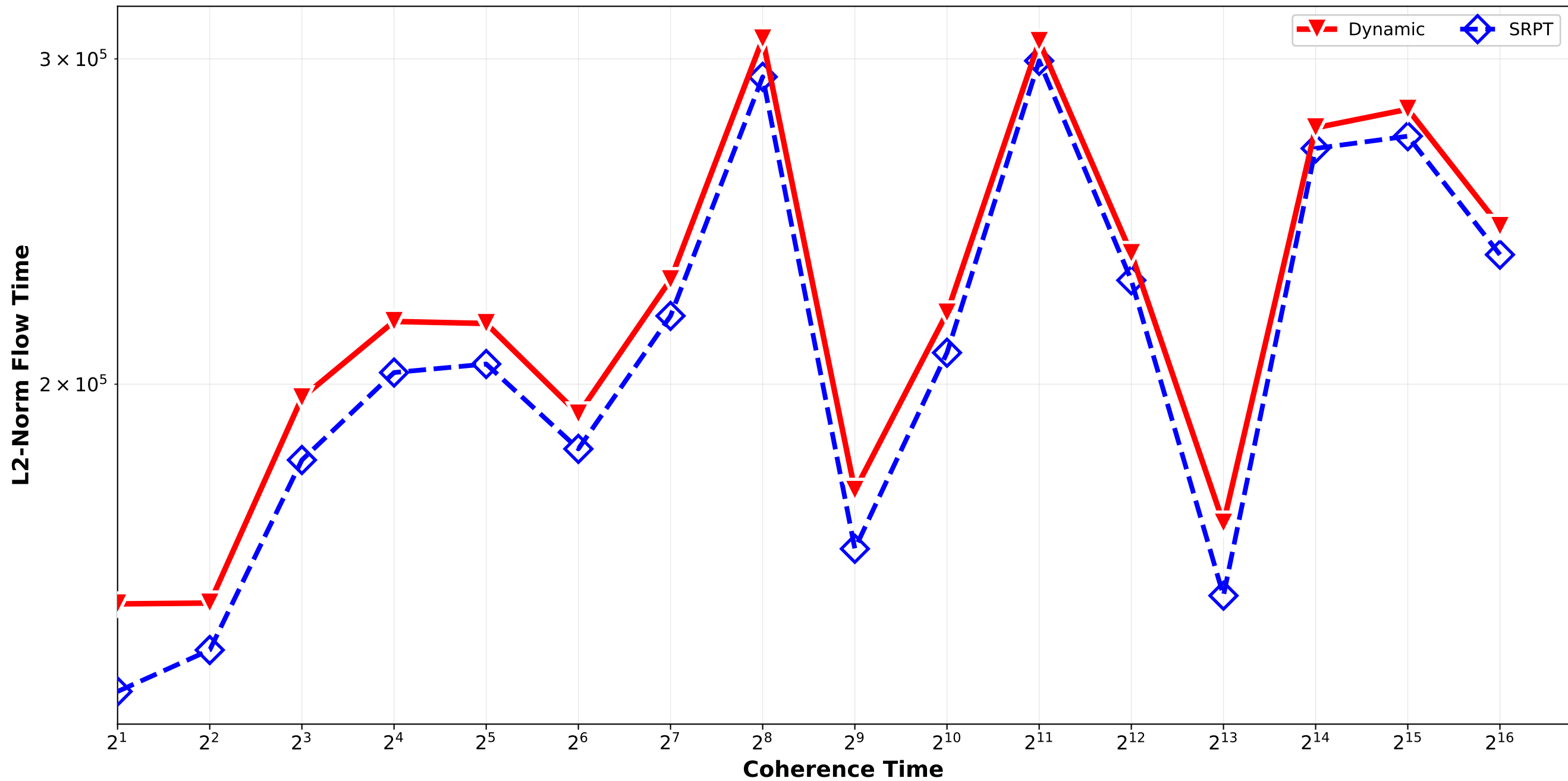
Dynamic vs SRPT - L2 Norm Flow Time Bounded_Pareto_combination_softrandom H32768_H262144 / pair_4
