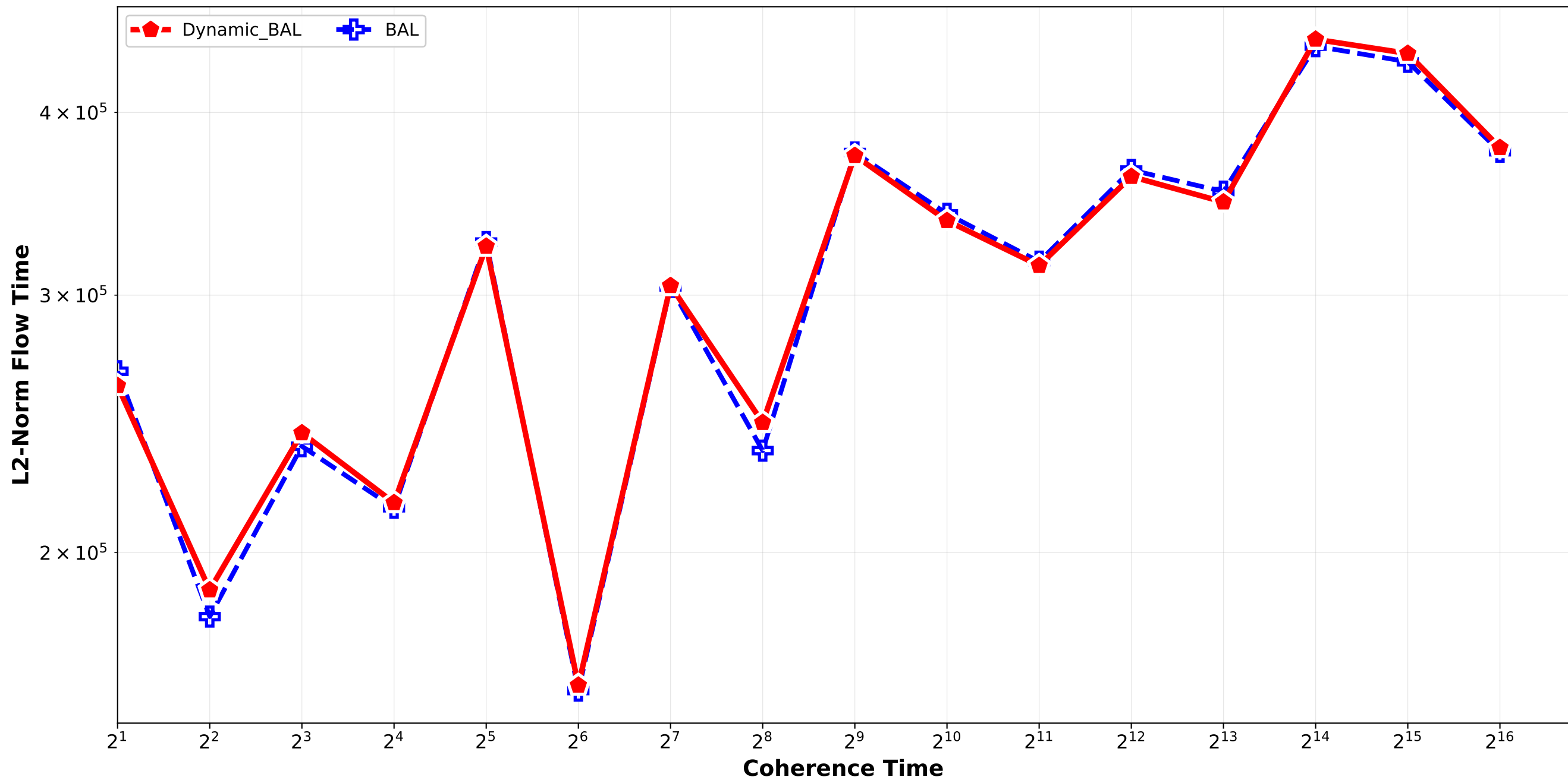
Dynamic_BAL vs BAL - L2 Norm Flow Time Bounded_Pareto_combination_softrandom H4096_H32768 / pair_3
