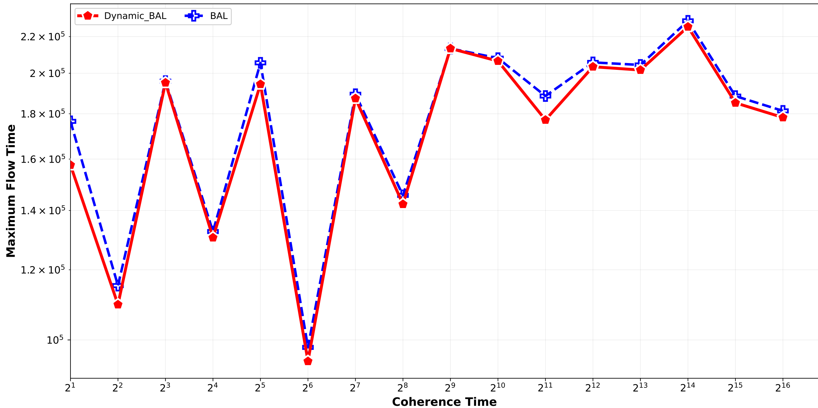
Dynamic_BAL vs BAL - Maximum Flow Time Bounded_Pareto_combination_softrandom H4096_H32768 / pair_3
