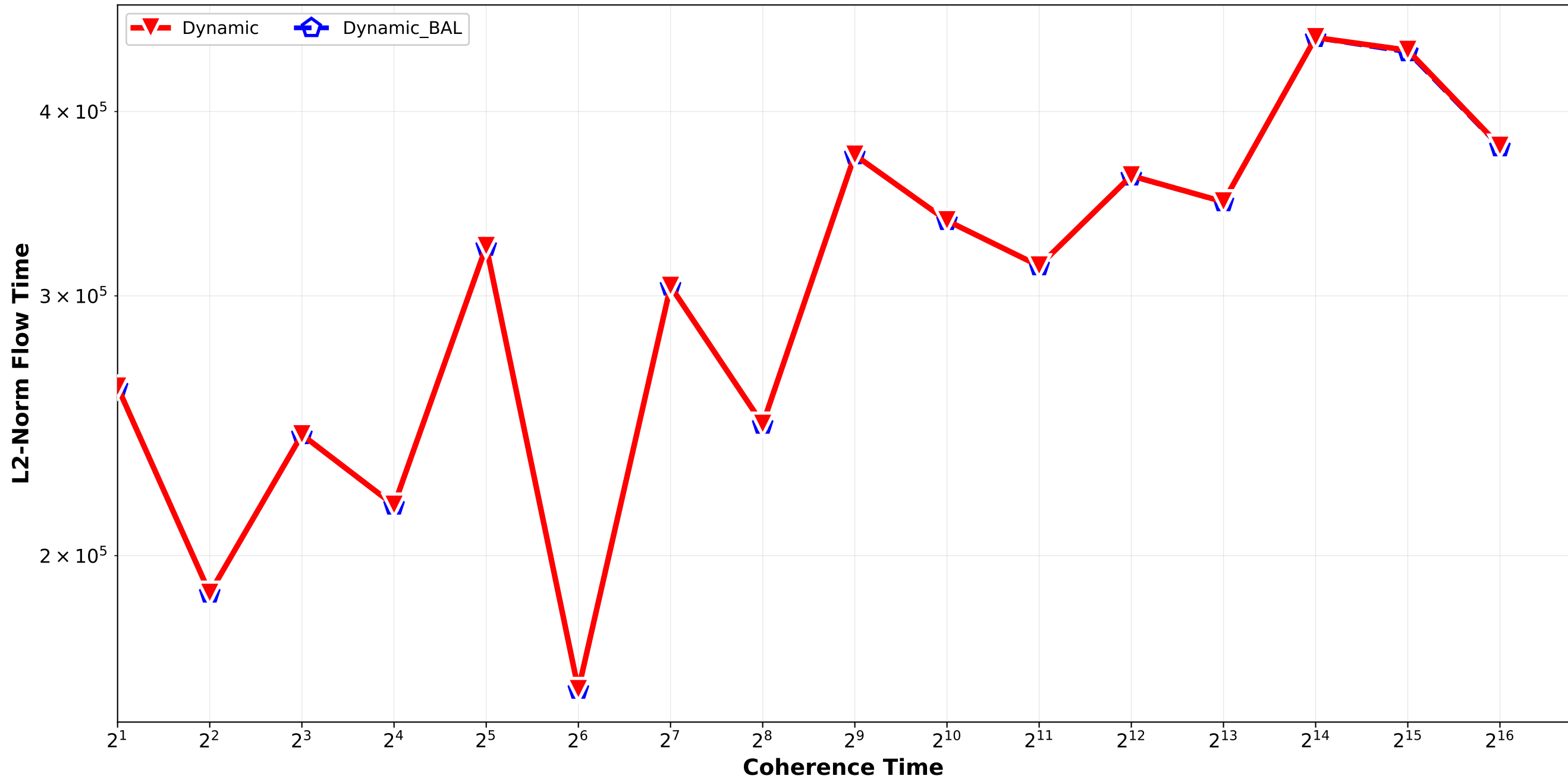
Dynamic vs Dynamic_BAL - L2 Norm Flow Time Bounded_Pareto_combination_softrandom H4096_H32768 / pair_3
