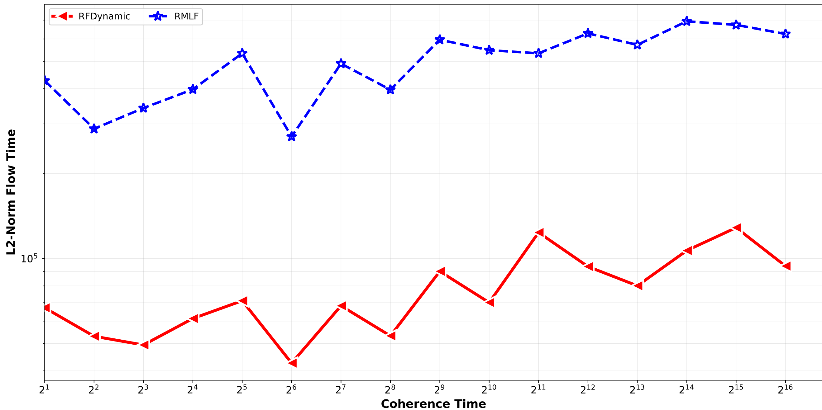
RFDynamic vs RMLF - L2 Norm Flow Time Bounded_Pareto_combination_softrandom H4096_H32768 / pair_3
