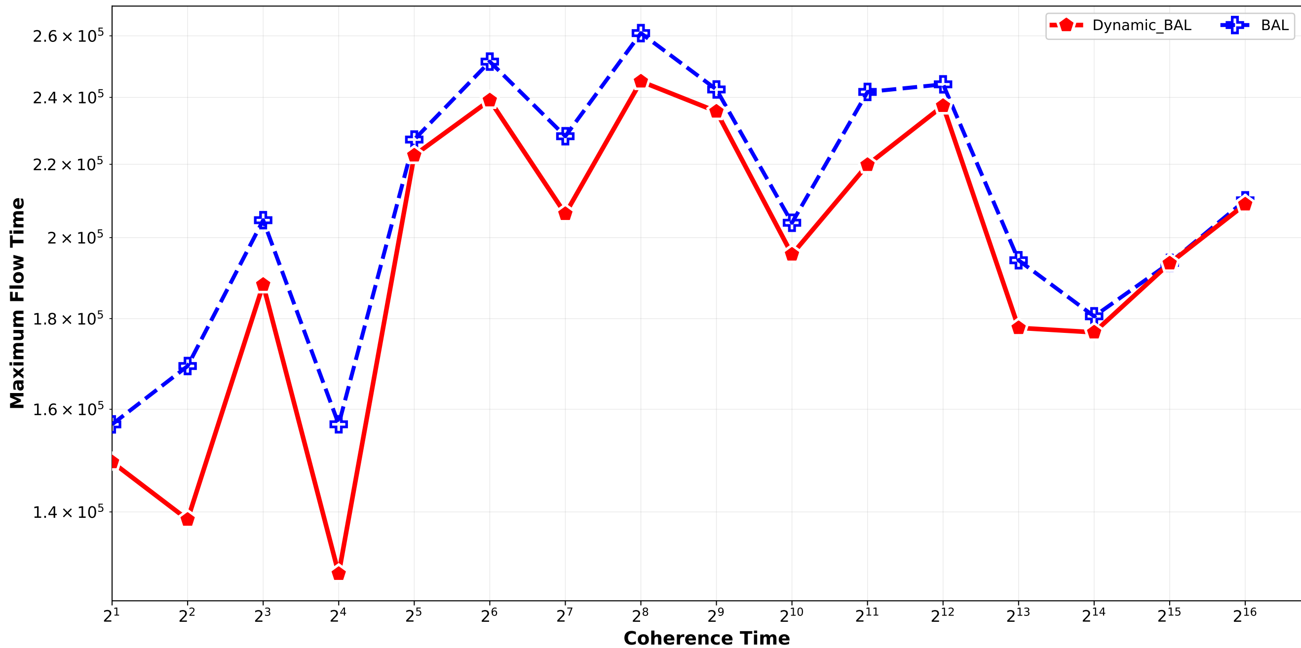
Dynamic_BAL vs BAL - Maximum Flow Time Bounded_Pareto_combination_softrandom H512_H4096 / pair_2
