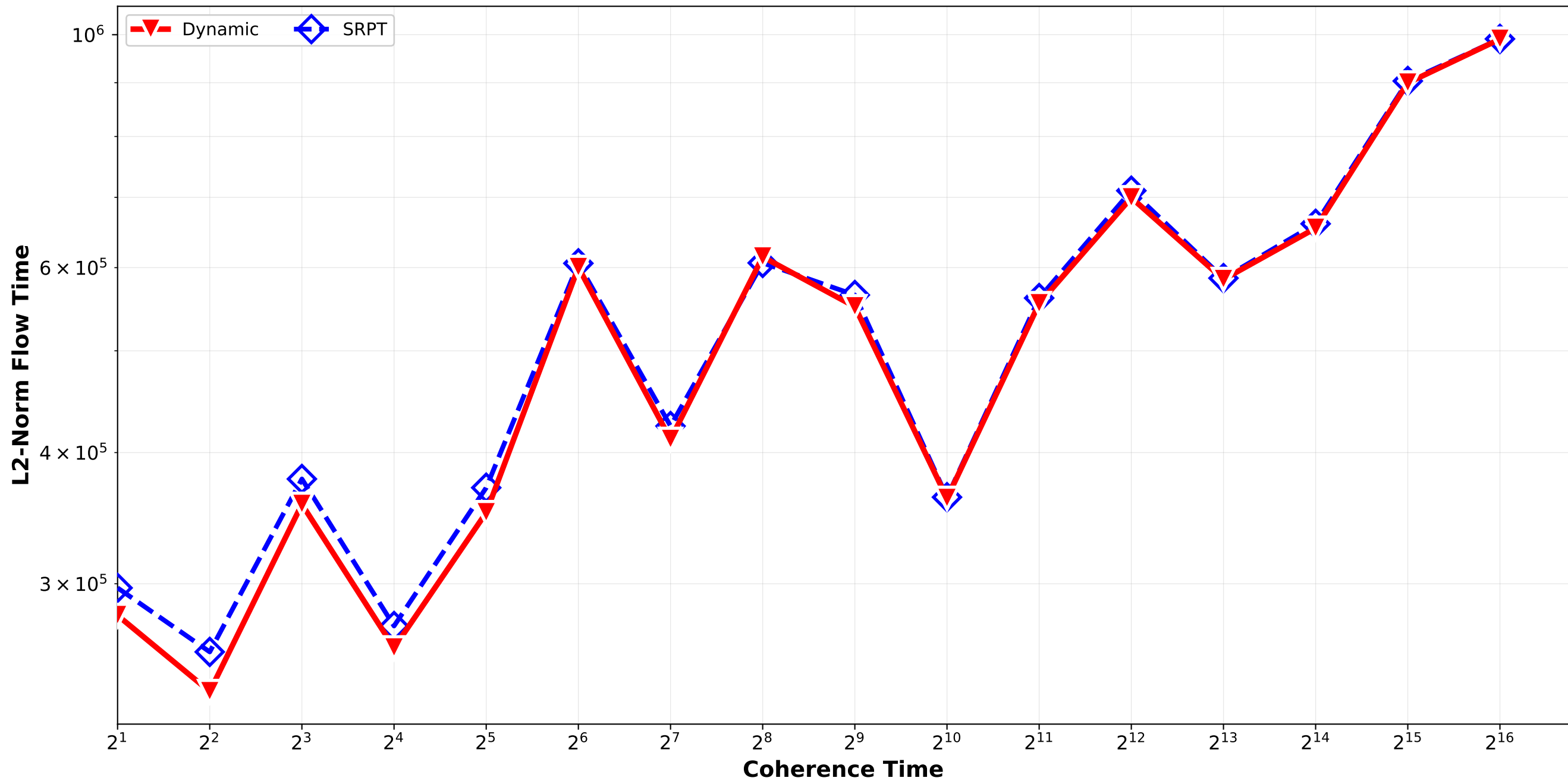
Dynamic vs SRPT - L2 Norm Flow Time Bounded_Pareto_combination_softrandom H512_H4096 / pair_2
