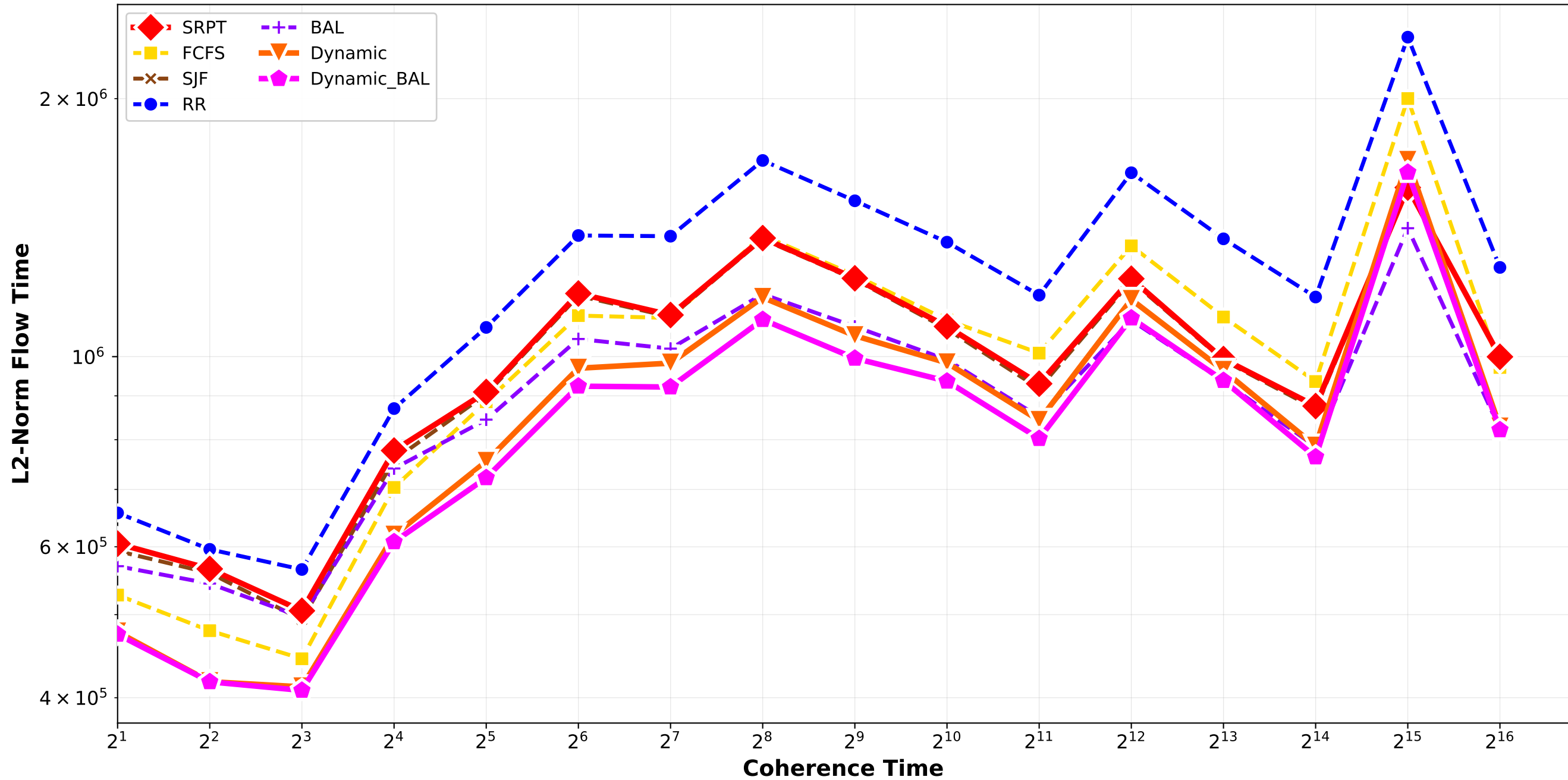
Clairvoyant Algorithms - L2 Norm Flow Time Bounded_Pareto_combination_softrandom H64_H512 / pair_1
