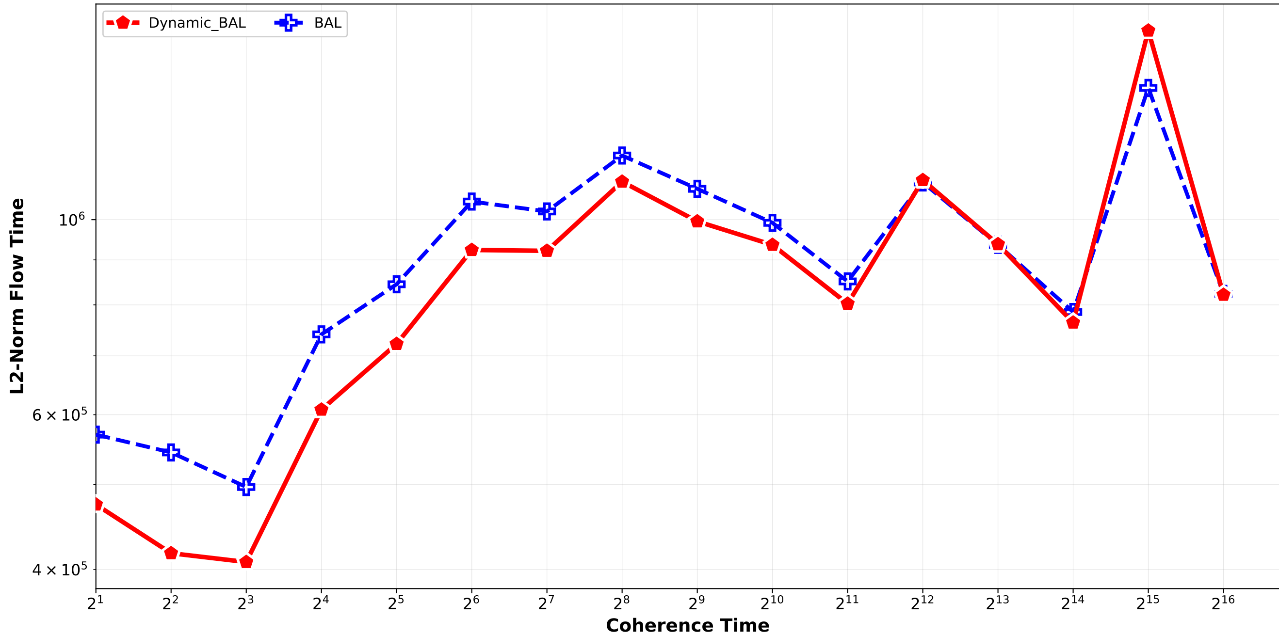
Dynamic_BAL vs BAL - L2 Norm Flow Time Bounded_Pareto_combination_softrandom H64_H512 / pair_1
