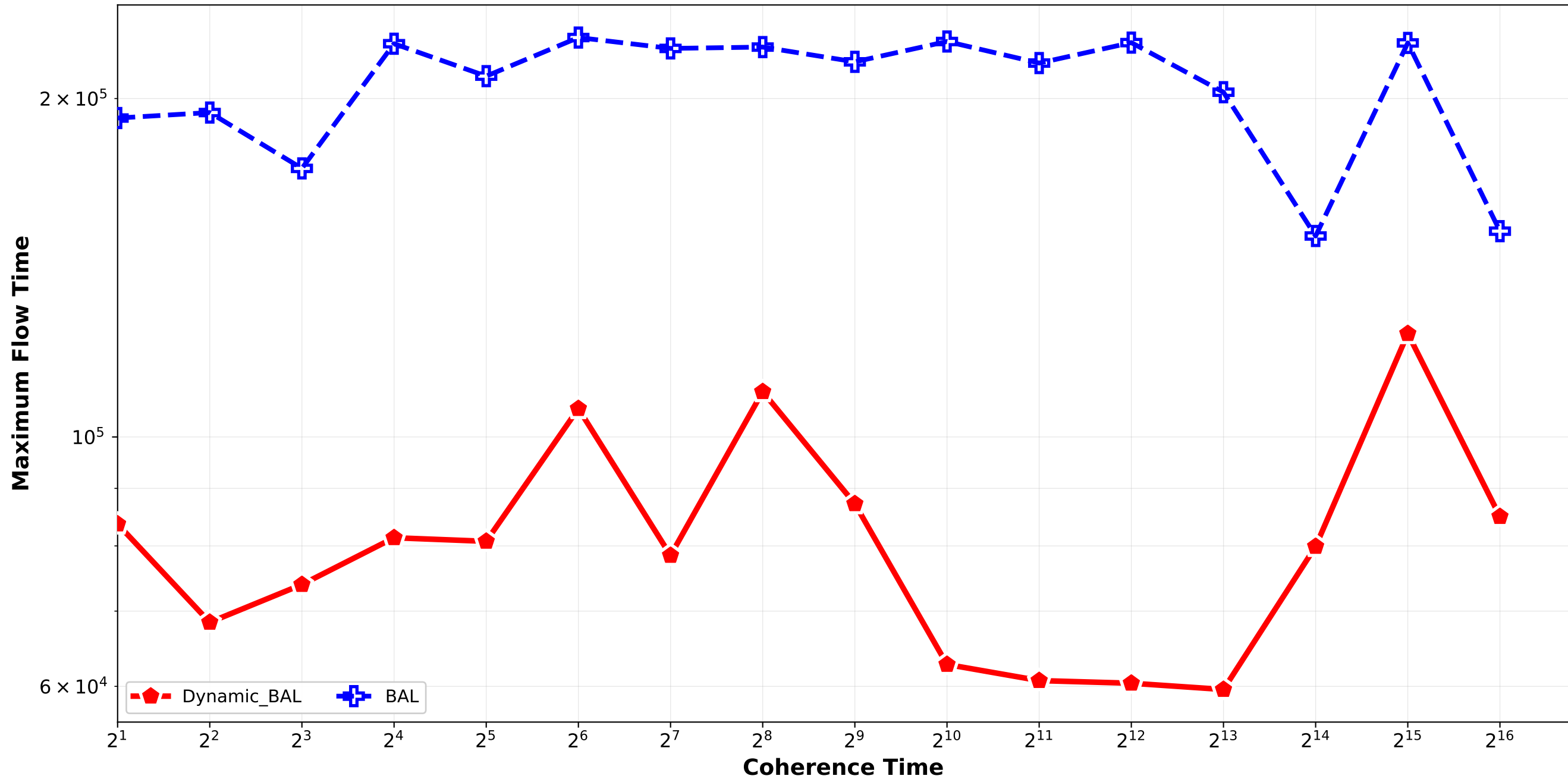
Dynamic_BAL vs BAL - Maximum Flow Time Bounded_Pareto_combination_softrandom H64_H512 / pair_1
