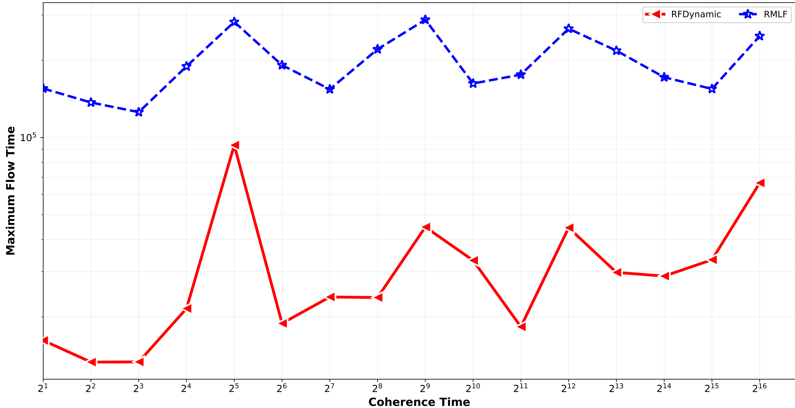
RFDynamic vs RMLF - Maximum Flow Time Bounded_Pareto_random
