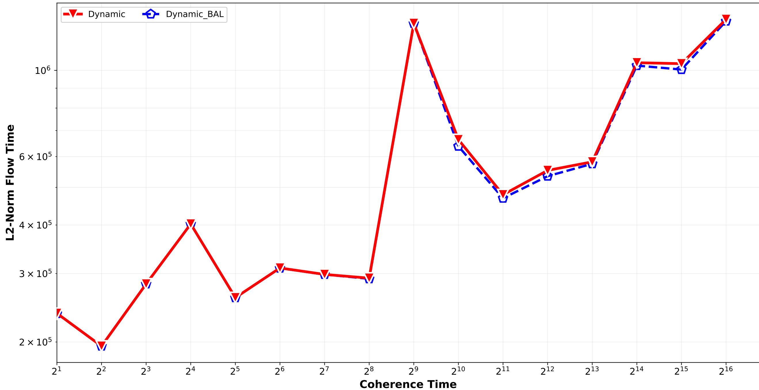
Dynamic vs Dynamic_BAL - L2 Norm Flow Time Bounded_Pareto_softrandom
