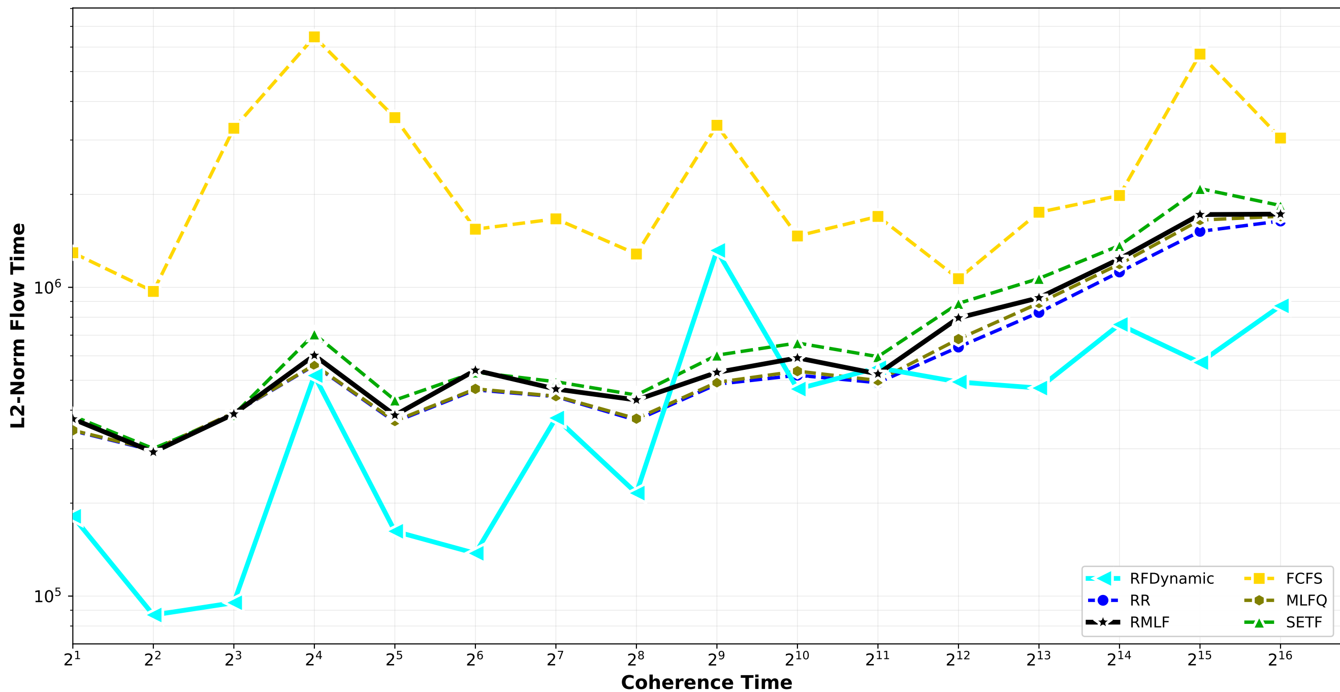
Non-Clairvoyant Algorithms - L2 Norm Flow Time Bounded_Pareto_softrandom
