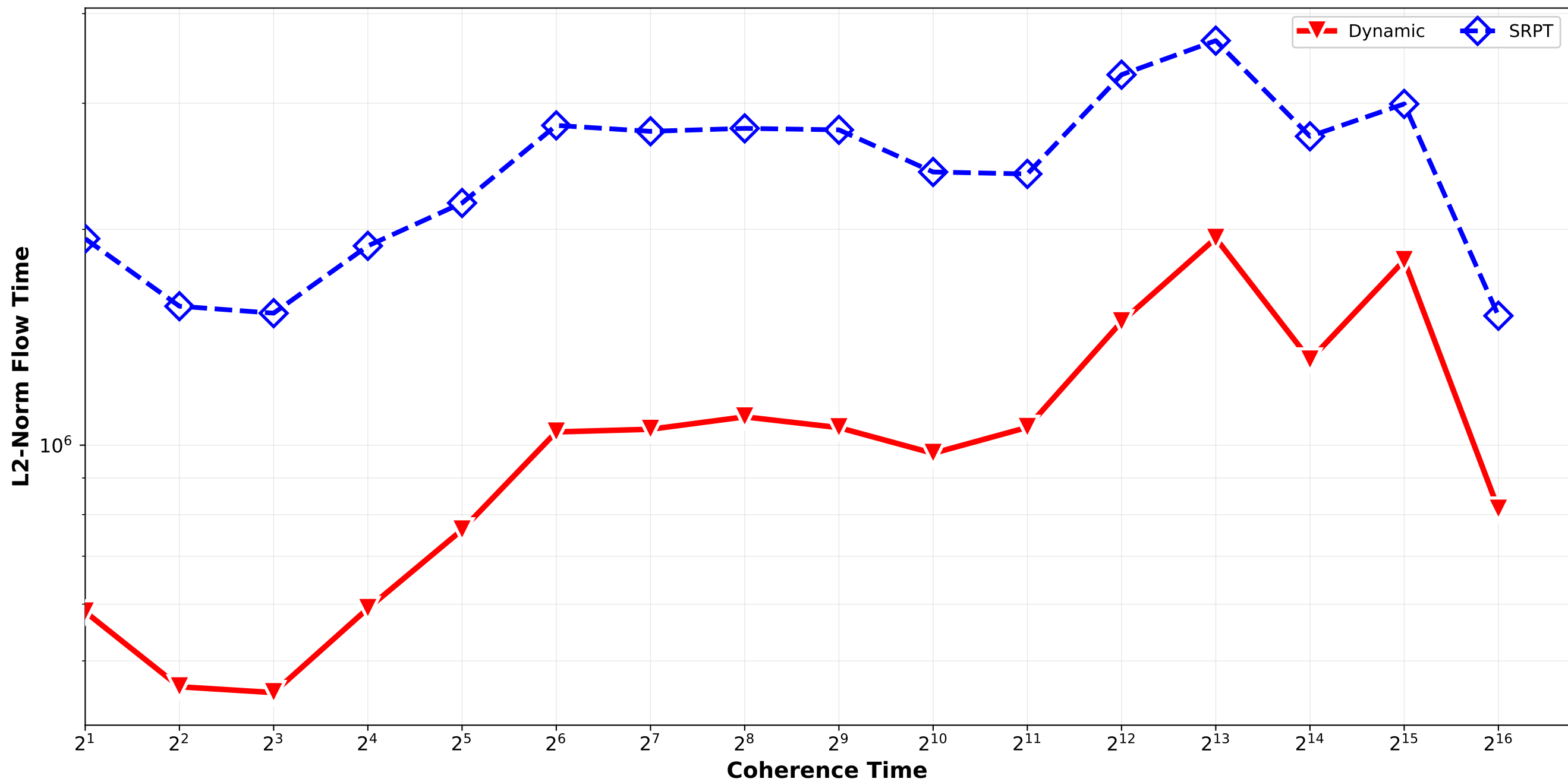
Dynamic vs SRPT - L2 Norm Flow Time normal_combination_random std6_std9_std12_std15 / quadruplet_1
