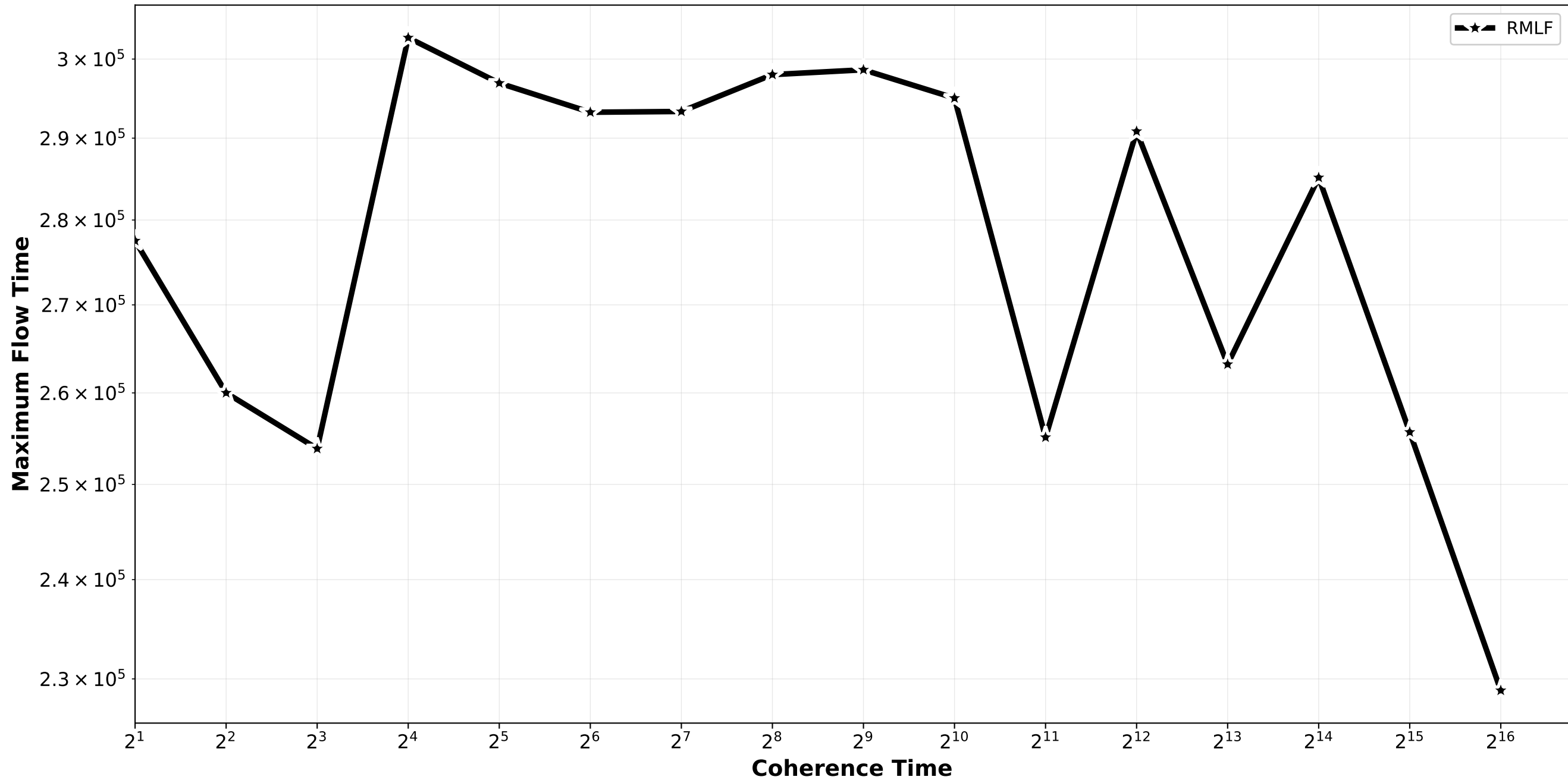
RFDynamic vs RMLF - Maximum Flow Time normal_combination_random std9_std12_std15_std18 / quadruplet_2
