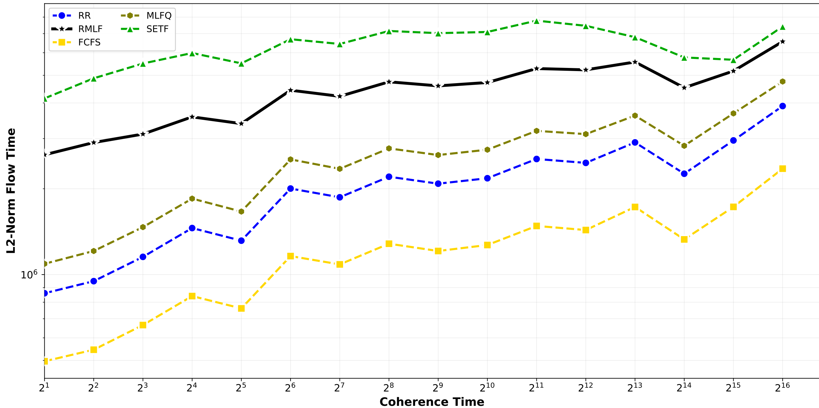
Non-Clairvoyant Algorithms - L2 Norm Flow Time normal_combination_random std12_std15_std18 / triplet_3
