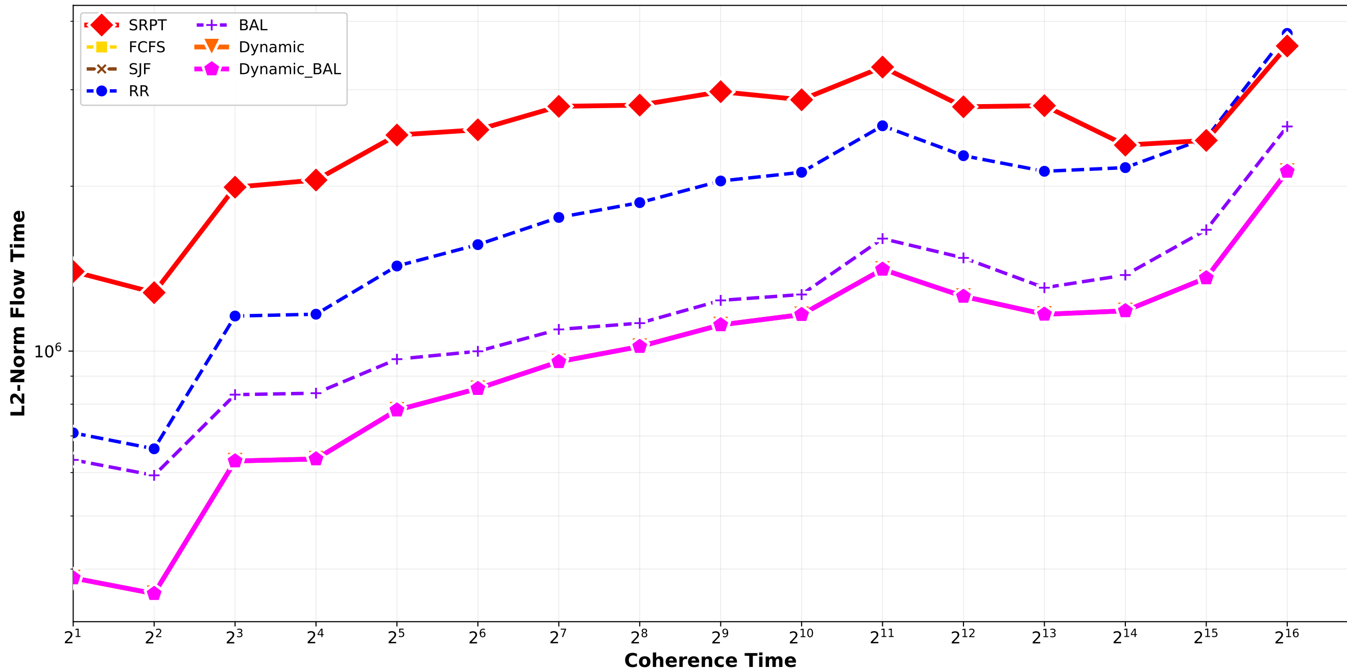
Clairvoyant Algorithms - L2 Norm Flow Time normal_combination_random std6_std9_std12 / triplet_1
