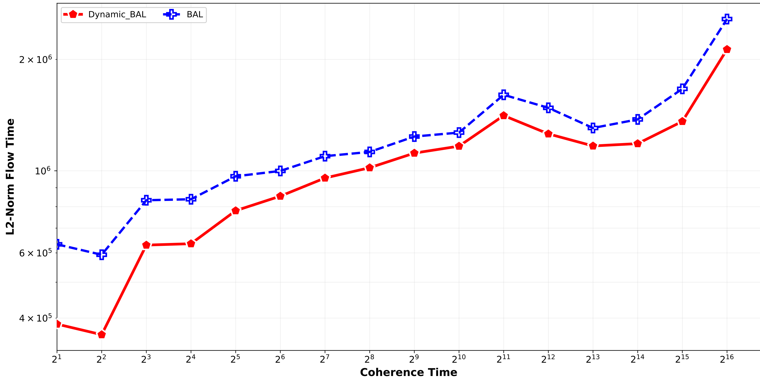
Dynamic_BAL vs BAL - L2 Norm Flow Time normal_combination_random std6_std9_std12 / triplet_1
