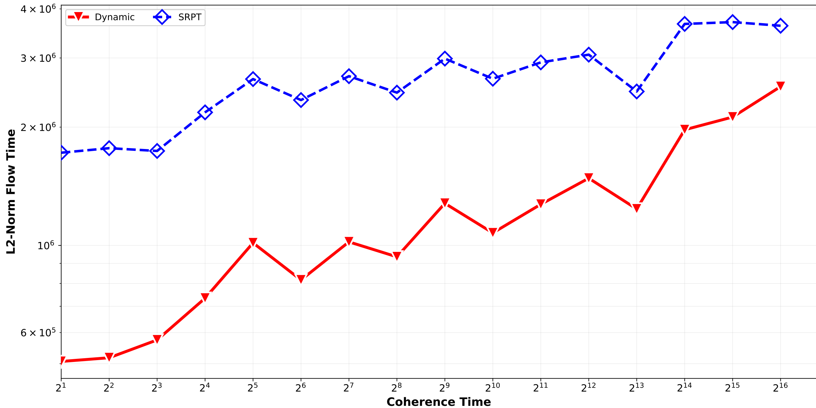
Dynamic vs SRPT - L2 Norm Flow Time normal_combination_random std9_std12_std15 / triplet_2
