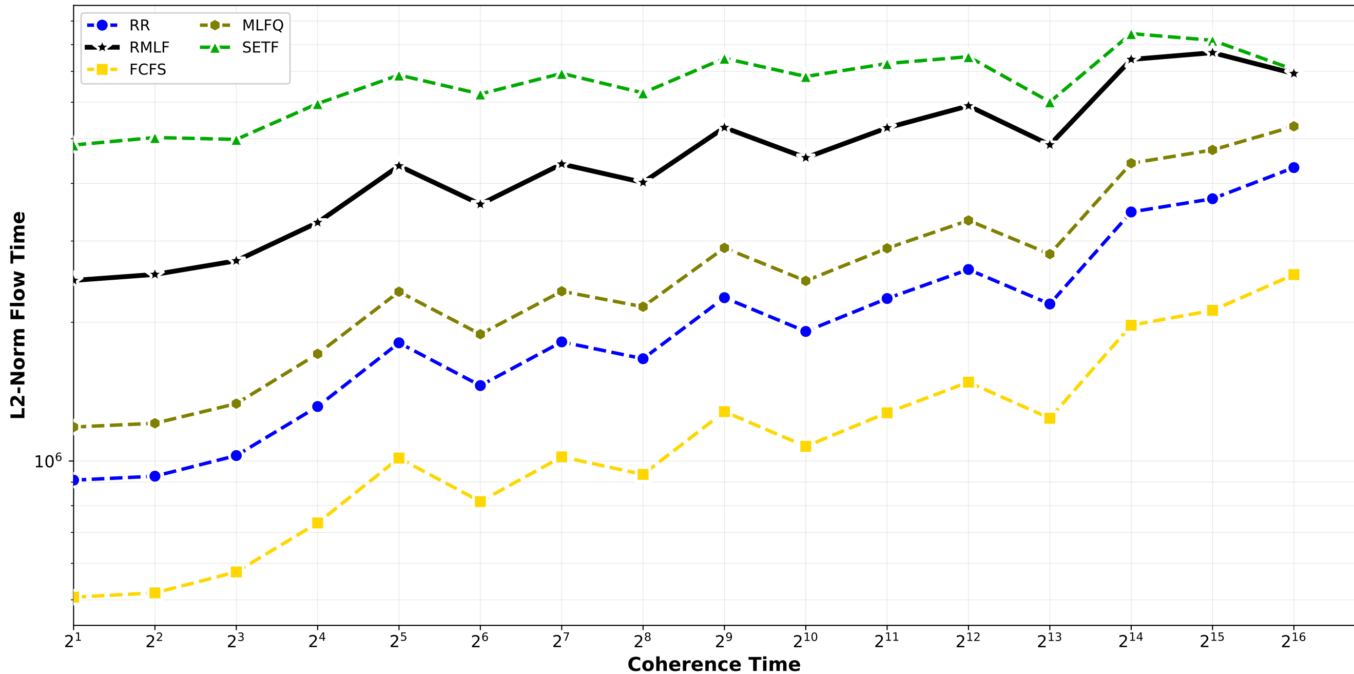
Non-Clairvoyant Algorithms - L2 Norm Flow Time normal_combination_random std9_std12_std15 / triplet_2
