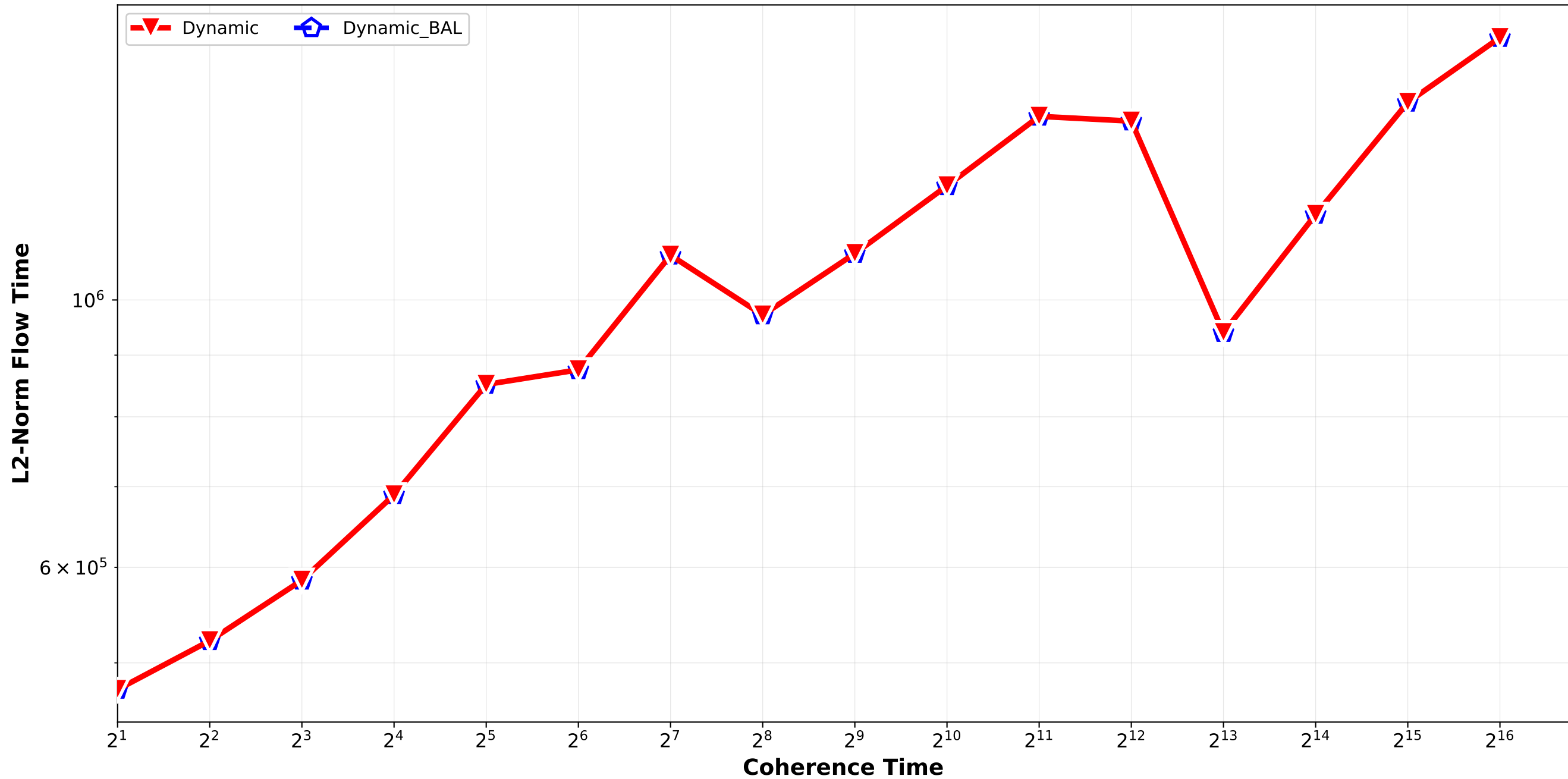
Dynamic vs Dynamic_BAL - L2 Norm Flow Time normal_combination_random std12_std15 / pair_3
