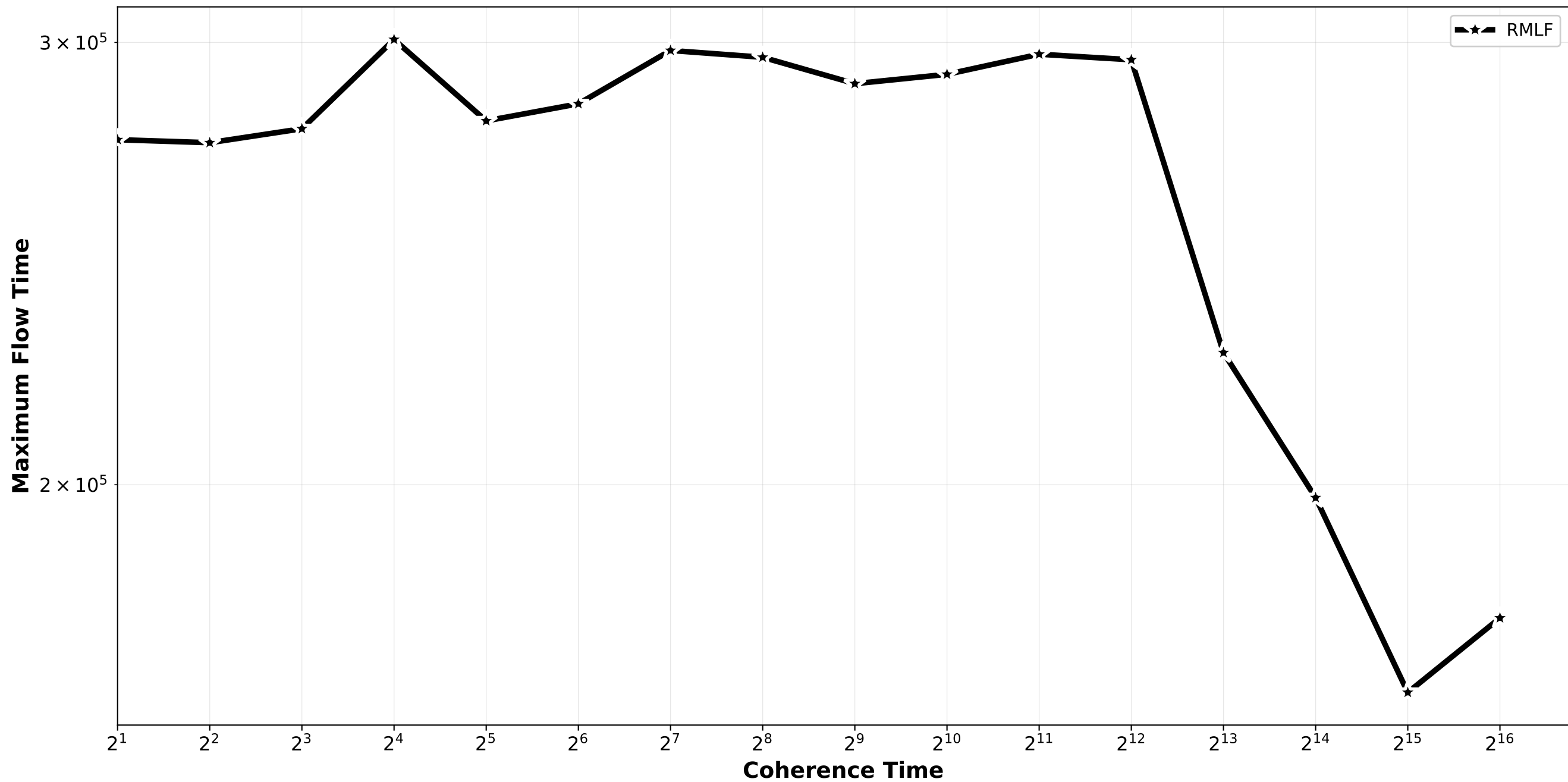
RFDynamic vs RMLF - Maximum Flow Time normal_combination_random std12_std15 / pair_3
