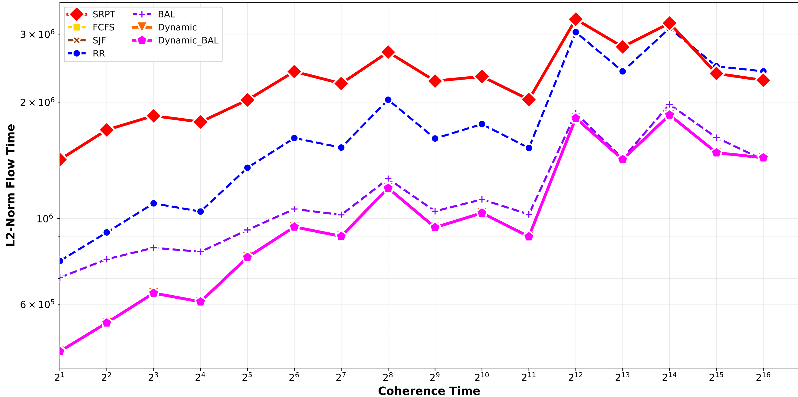
Clairvoyant Algorithms - L2 Norm Flow Time normal_combination_random std15_std18 / pair_4
