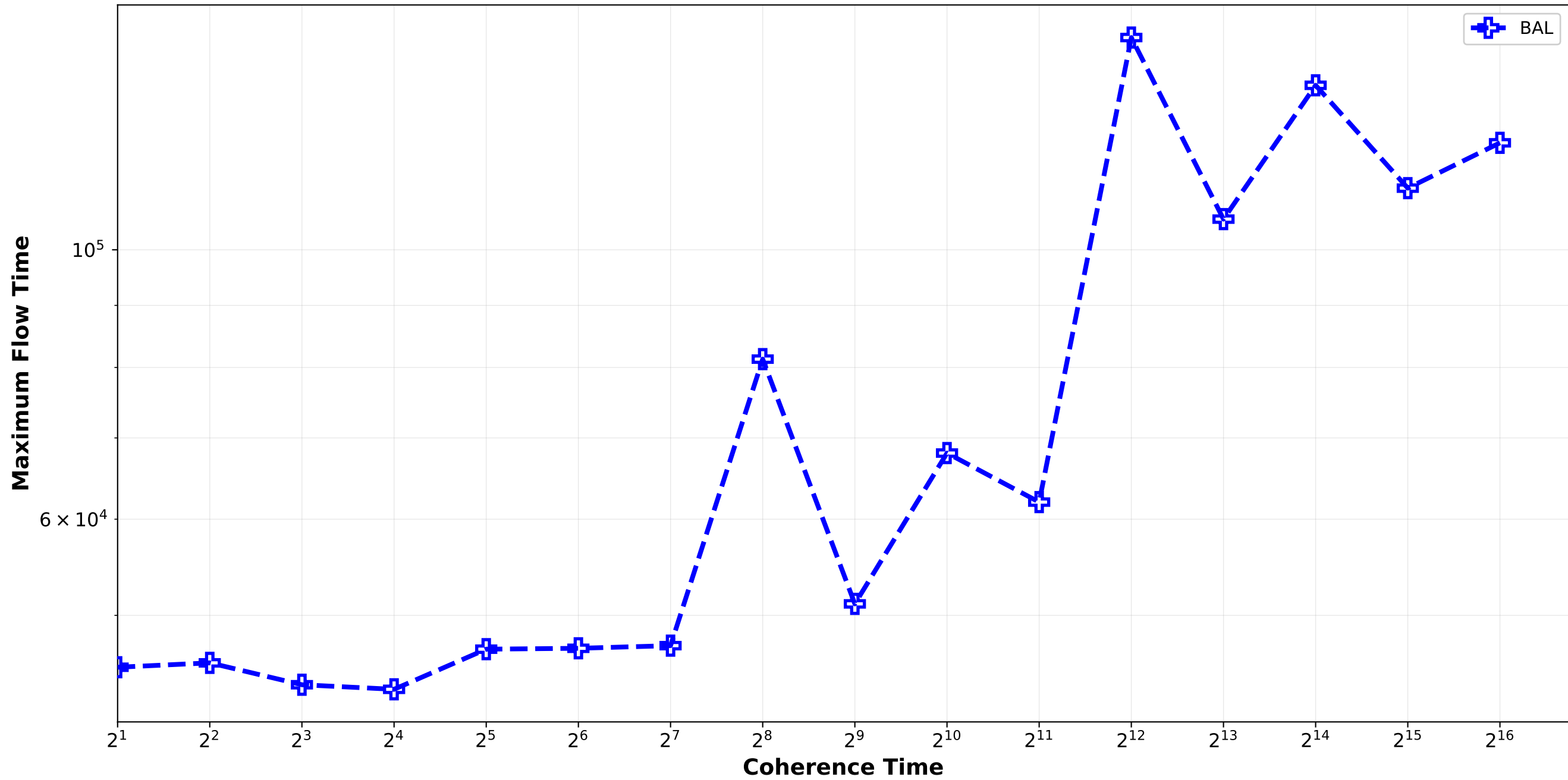
Dynamic_BAL vs BAL - Maximum Flow Time normal_combination_random std15_std18 / pair_4
